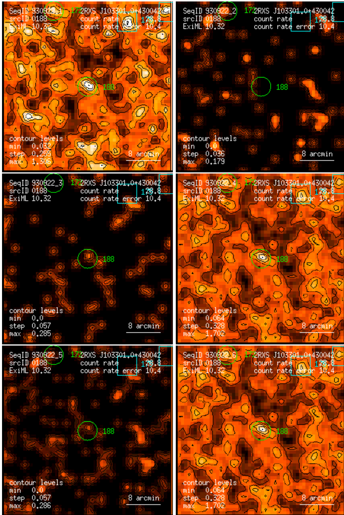
Figure 188: RASS 930922: detection 0188: band rate images, Gaussian filter: (1) PSPC channels 11 – 41, (2) 52 – 90, (3) 91 – 201, (4) 11 – 235, (5) 52 – 201, (6) 11 – 201. Broad band rates in counts/ks. Band rate contour levels in counts/ks/arcmin 2 .
