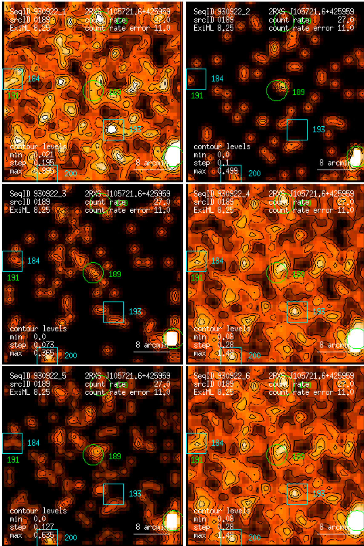
Figure 189: RASS 930922: detection 0189: band rate images, Gaussian filter: (1) PSPC channels 11 – 41, (2) 52 – 90, (3) 91 – 201, (4) 11 – 235, (5) 52 – 201, (6) 11 – 201. Broad band rates in counts/ks. Band rate contour levels in counts/ks/arcmin 2 .
