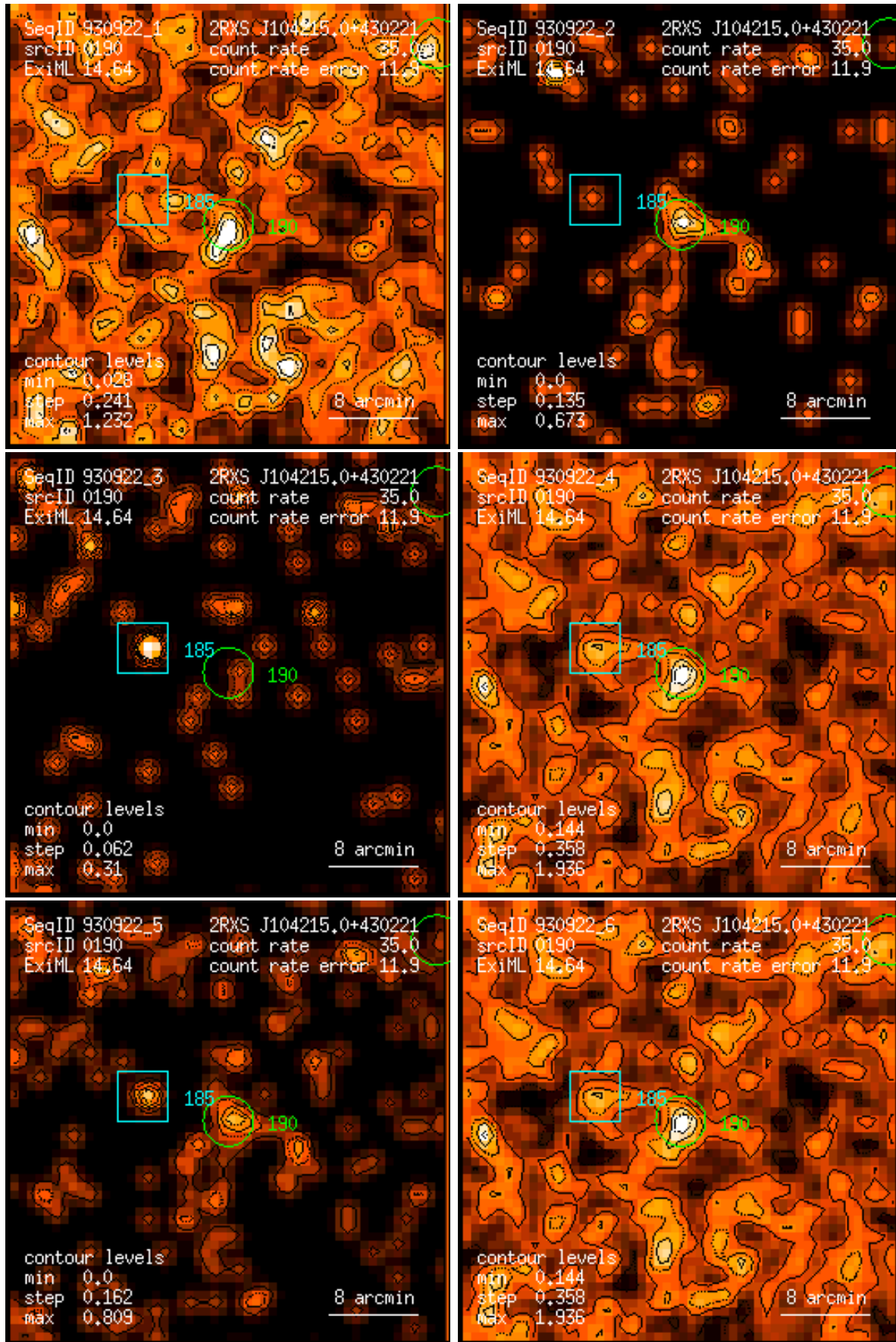
Figure 190: RASS 930922: detection 0190: band rate images, Gaussian filter: (1) PSPC channels 11 – 41, (2) 52 – 90, (3) 91 – 201, (4) 11 – 235, (5) 52 – 201, (6) 11 – 201. Broad band rates in counts/ks. Band rate contour levels in counts/ks/arcmin 2 .
