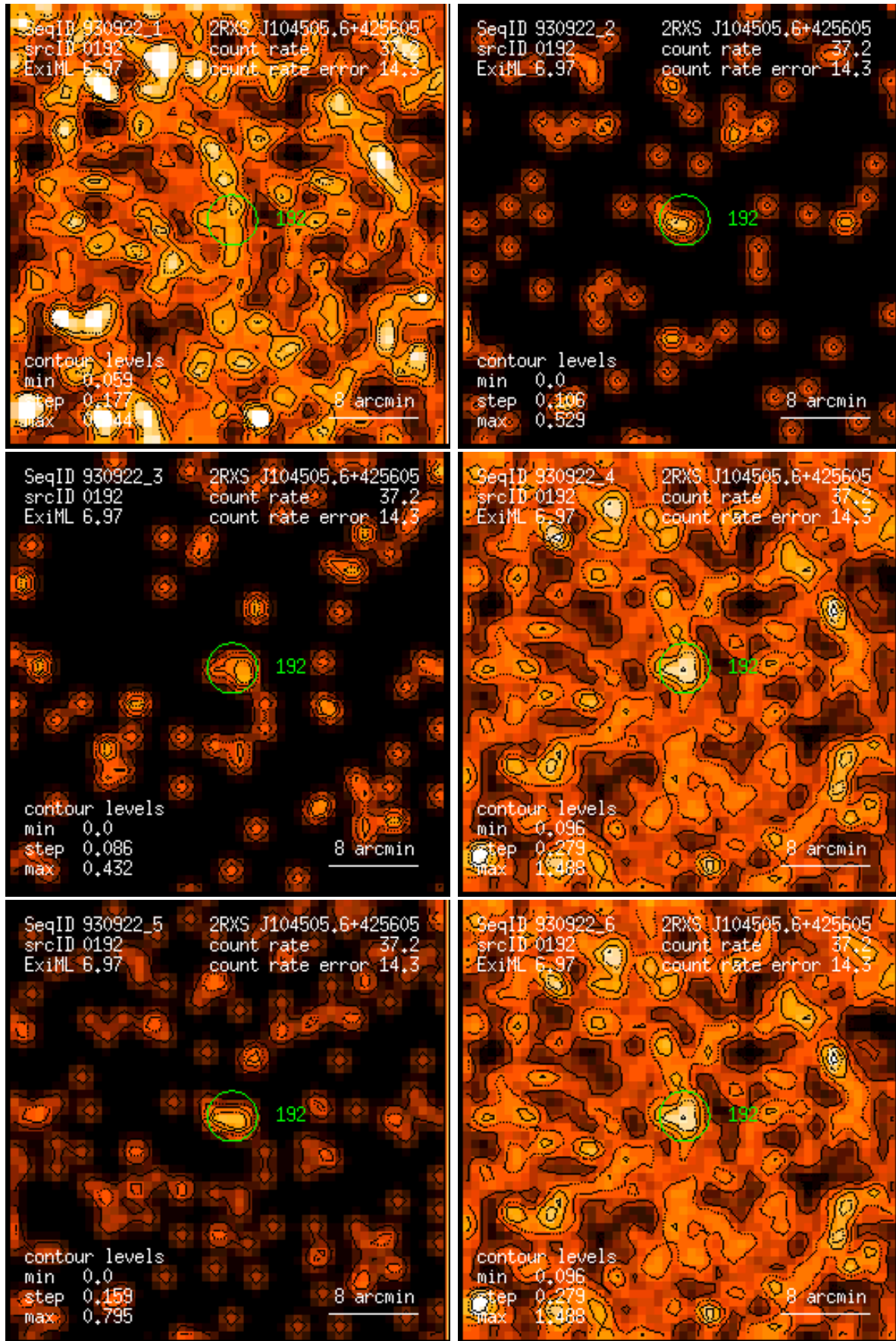
Figure 192: RASS 930922: detection 0192: band rate images, Gaussian filter: (1) PSPC channels 11 – 41, (2) 52 – 90, (3) 91 – 201, (4) 11 – 235, (5) 52 – 201, (6) 11 – 201. Broad band rates in counts/ks. Band rate contour levels in counts/ks/arcmin 2 .
