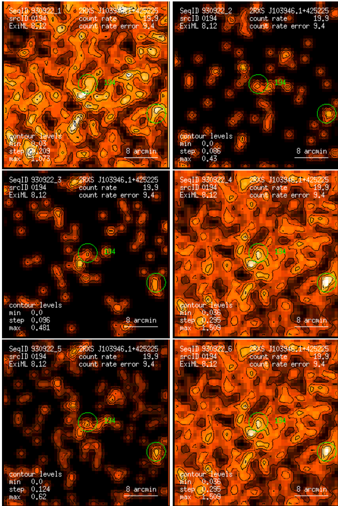
Figure 194: RASS 930922: detection 0194: band rate images, Gaussian filter: (1) PSPC channels 11 – 41, (2) 52 – 90, (3) 91 – 201, (4) 11 – 235, (5) 52 – 201, (6) 11 – 201. Broad band rates in counts/ks. Band rate contour levels in counts/ks/arcmin 2 .
