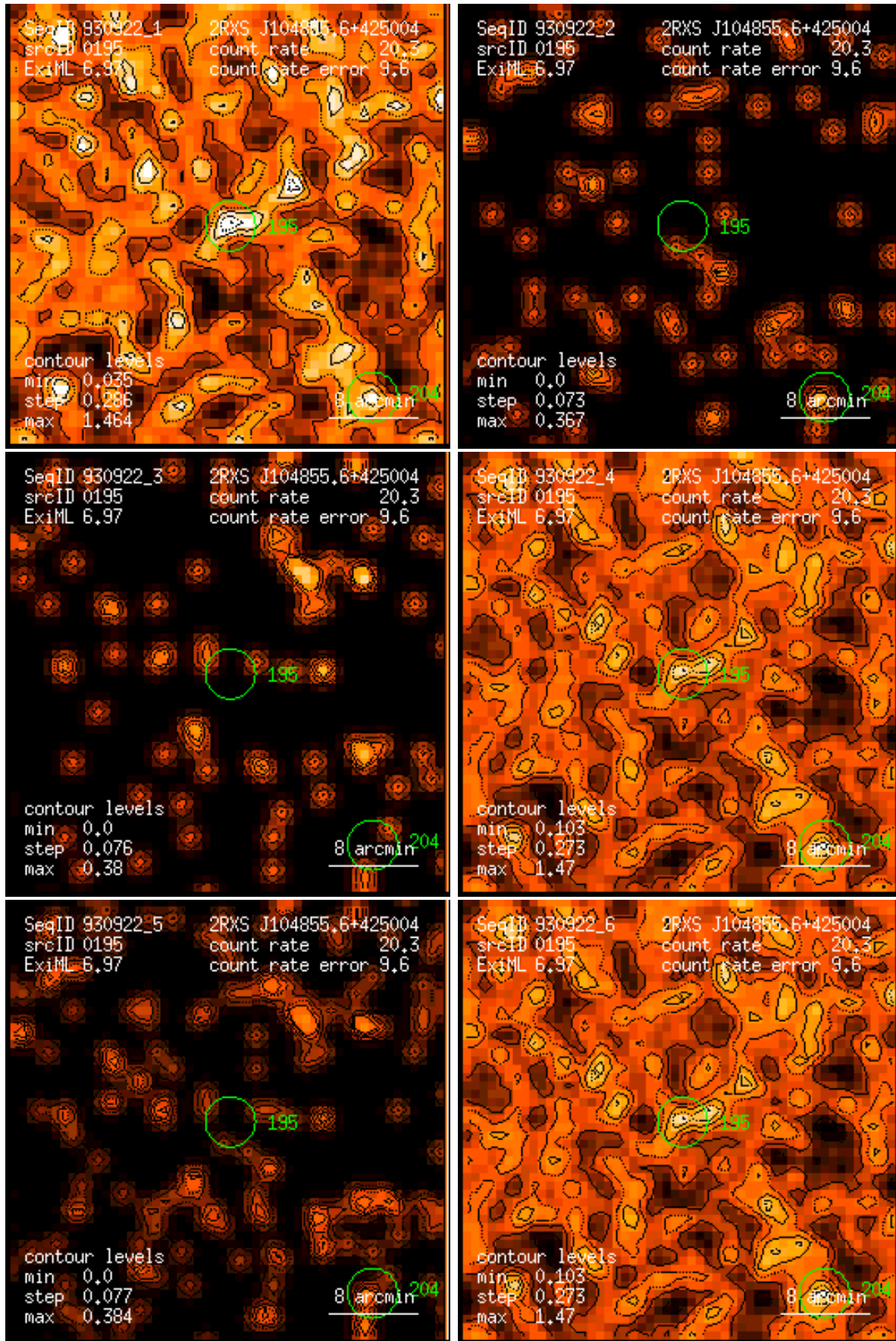
Figure 195: RASS 930922: detection 0195: band rate images, Gaussian filter: (1) PSPC channels 11 – 41, (2) 52 – 90, (3) 91 – 201, (4) 11 – 235, (5) 52 – 201, (6) 11 – 201. Broad band rates in counts/ks. Band rate contour levels in counts/ks/arcmin 2 .
