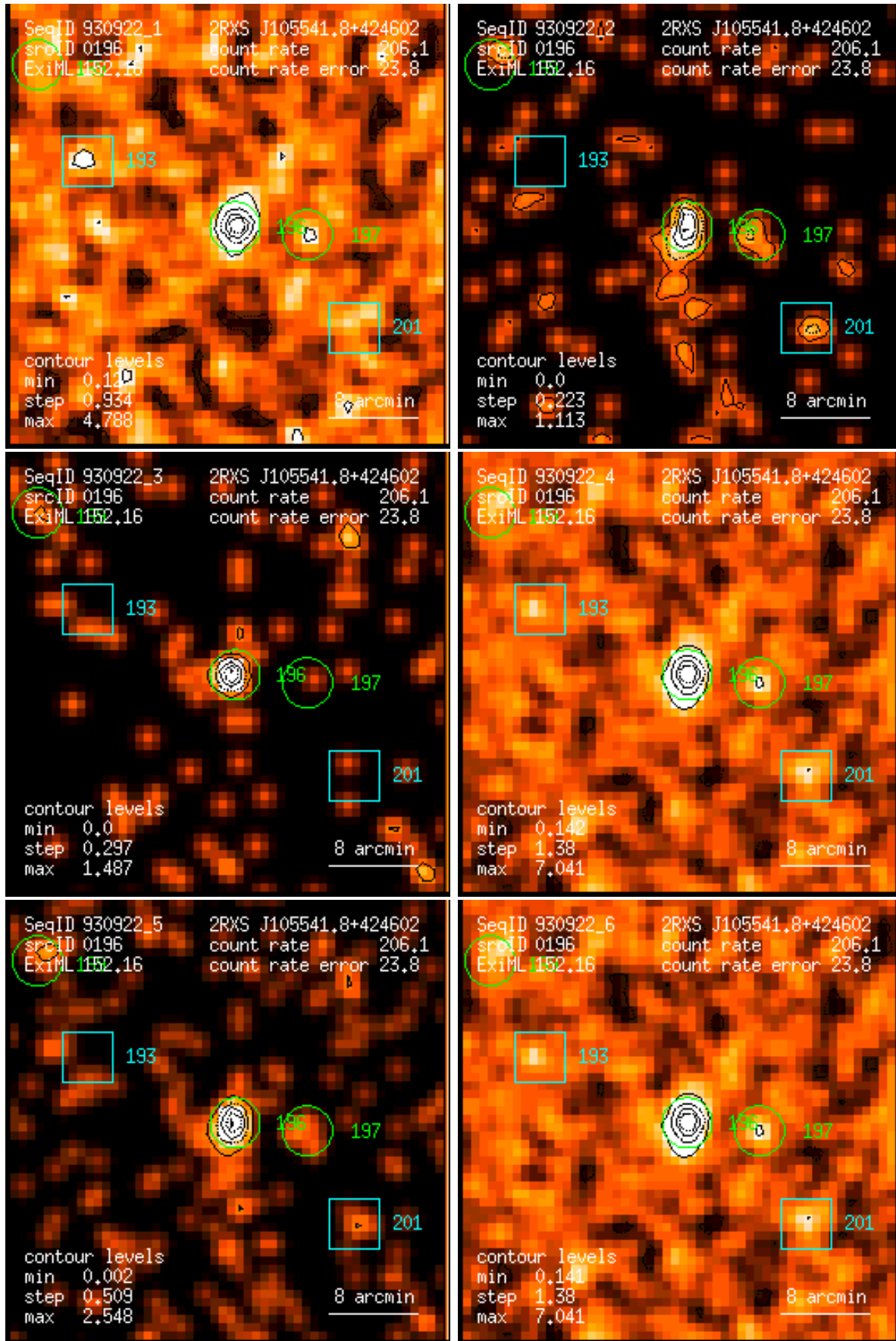
Figure 196: RASS 930922: detection 0196: band rate images, Gaussian filter: (1) PSPC channels 11 – 41, (2) 52 – 90, (3) 91 – 201, (4) 11 – 235, (5) 52 – 201, (6) 11 – 201. Broad band rates in counts/ks. Band rate contour levels in counts/ks/arcmin 2 .
