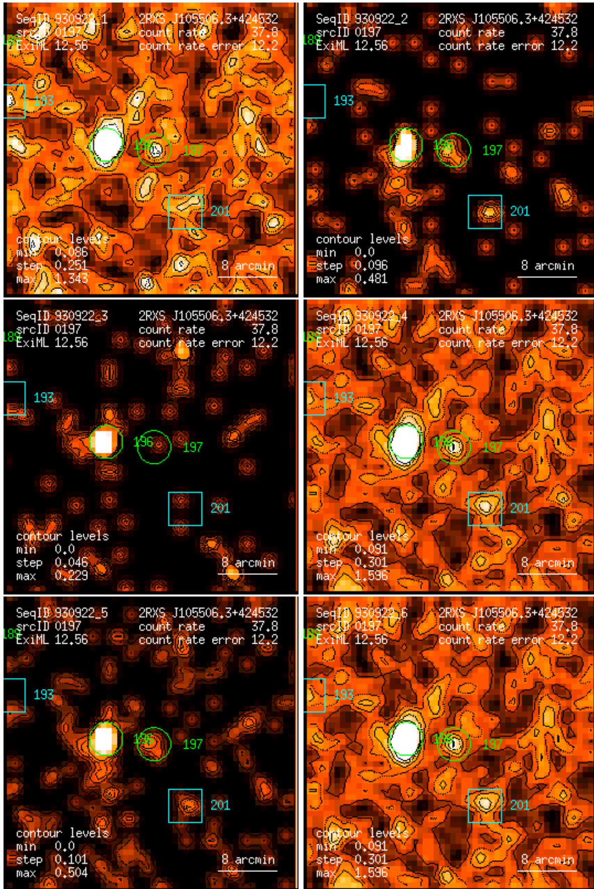
Figure 197: RASS 930922: detection 0197: band rate images, Gaussian filter: (1) PSPC channels 11 – 41, (2) 52 – 90, (3) 91 – 201, (4) 11 – 235, (5) 52 – 201, (6) 11 – 201. Broad band rates in counts/ks. Band rate contour levels in counts/ks/arcmin 2 .
