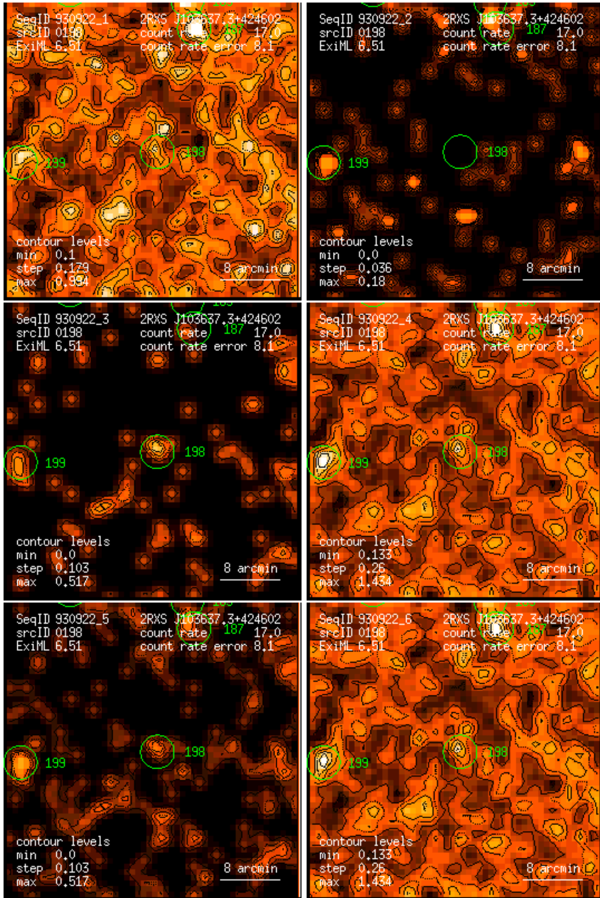
Figure 198: RASS 930922: detection 0198: band rate images, Gaussian filter: (1) PSPC channels 11 – 41, (2) 52 – 90, (3) 91 – 201, (4) 11 – 235, (5) 52 – 201, (6) 11 – 201. Broad band rates in counts/ks. Band rate contour levels in counts/ks/arcmin 2 .
