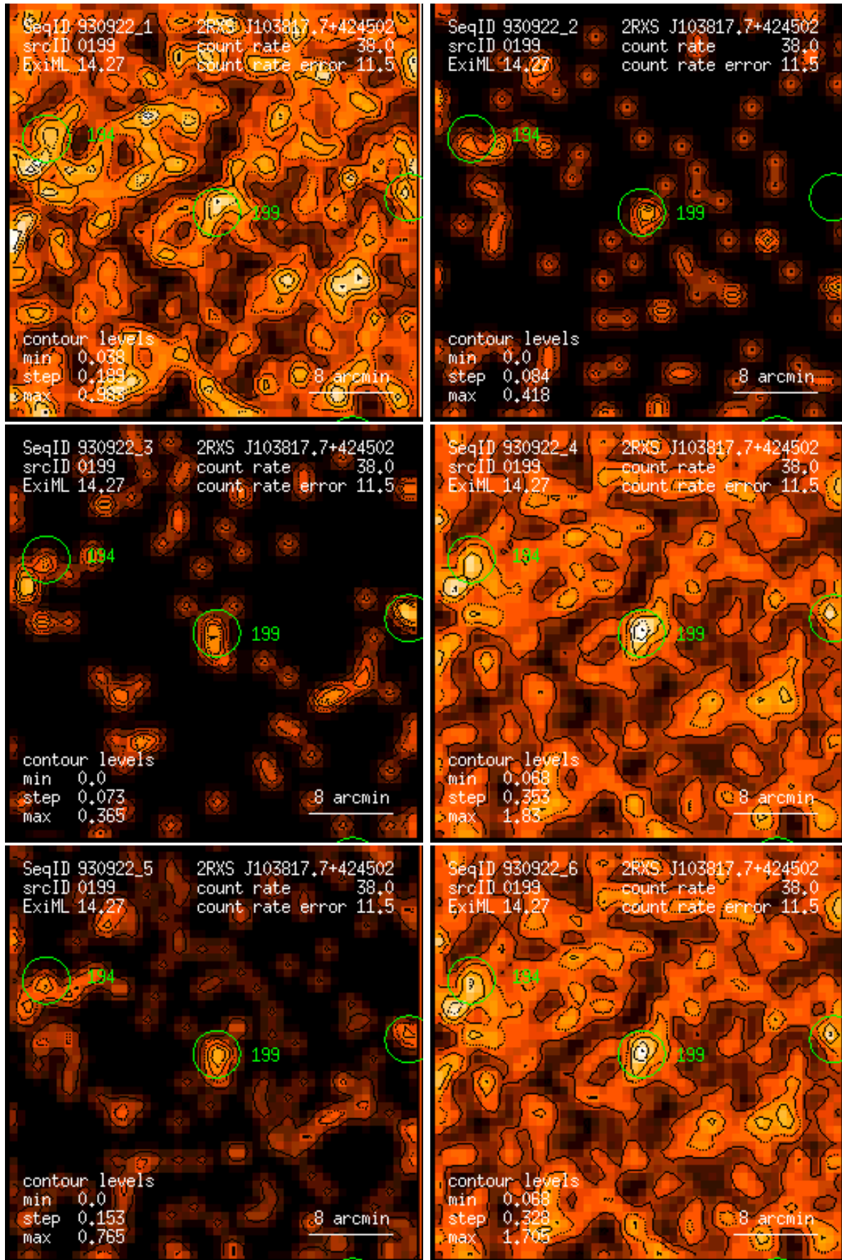
Figure 199: RASS 930922: detection 0199: band rate images, Gaussian filter: (1) PSPC channels 11 – 41, (2) 52 – 90, (3) 91 – 201, (4) 11 – 235, (5) 52 – 201, (6) 11 – 201. Broad band rates in counts/ks. Band rate contour levels in counts/ks/arcmin 2 .
