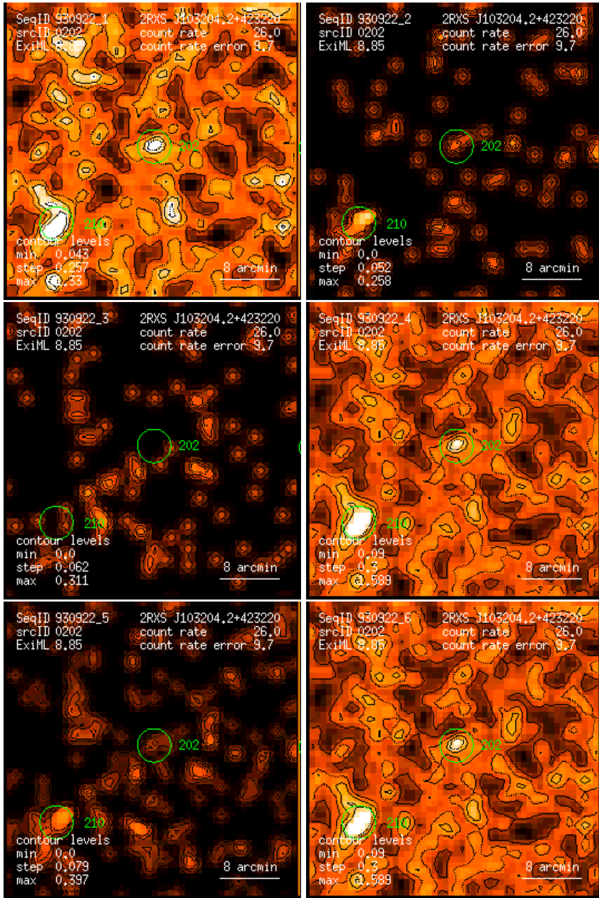
Figure 202: RASS 930922: detection 0202: band rate images, Gaussian filter: (1) PSPC channels 11 – 41, (2) 52 – 90, (3) 91 – 201, (4) 11 – 235, (5) 52 – 201, (6) 11 – 201. Broad band rates in counts/ks. Band rate contour levels in counts/ks/arcmin 2 .
