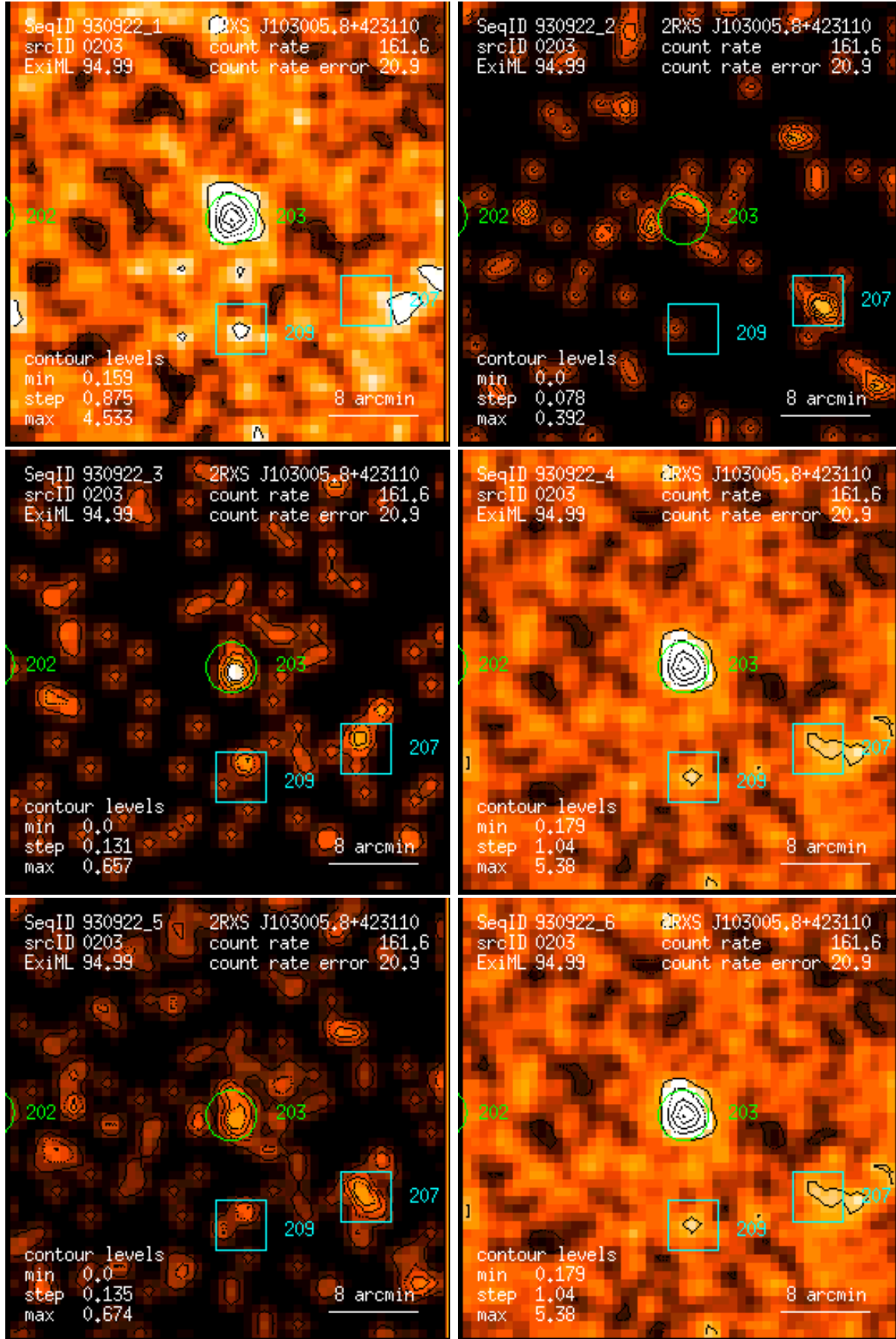
Figure 203: RASS 930922: detection 0203: band rate images, Gaussian filter: (1) PSPC channels 11 – 41, (2) 52 – 90, (3) 91 – 201, (4) 11 – 235, (5) 52 – 201, (6) 11 – 201. Broad band rates in counts/ks. Band rate contour levels in counts/ks/arcmin 2 .
