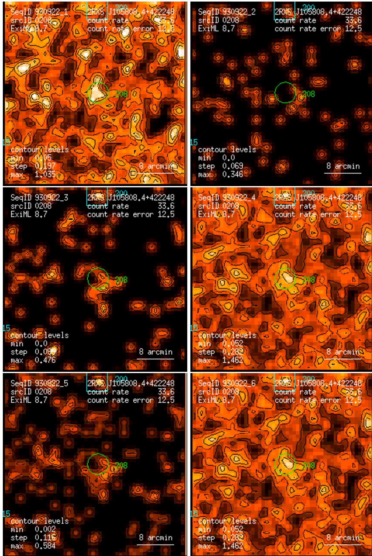
Figure 208: RASS 930922: detection 0208: band rate images, Gaussian filter: (1) PSPC channels 11 – 41, (2) 52 – 90, (3) 91 – 201, (4) 11 – 235, (5) 52 – 201, (6) 11 – 201. Broad band rates in counts/ks. Band rate contour levels in counts/ks/arcmin 2 .
