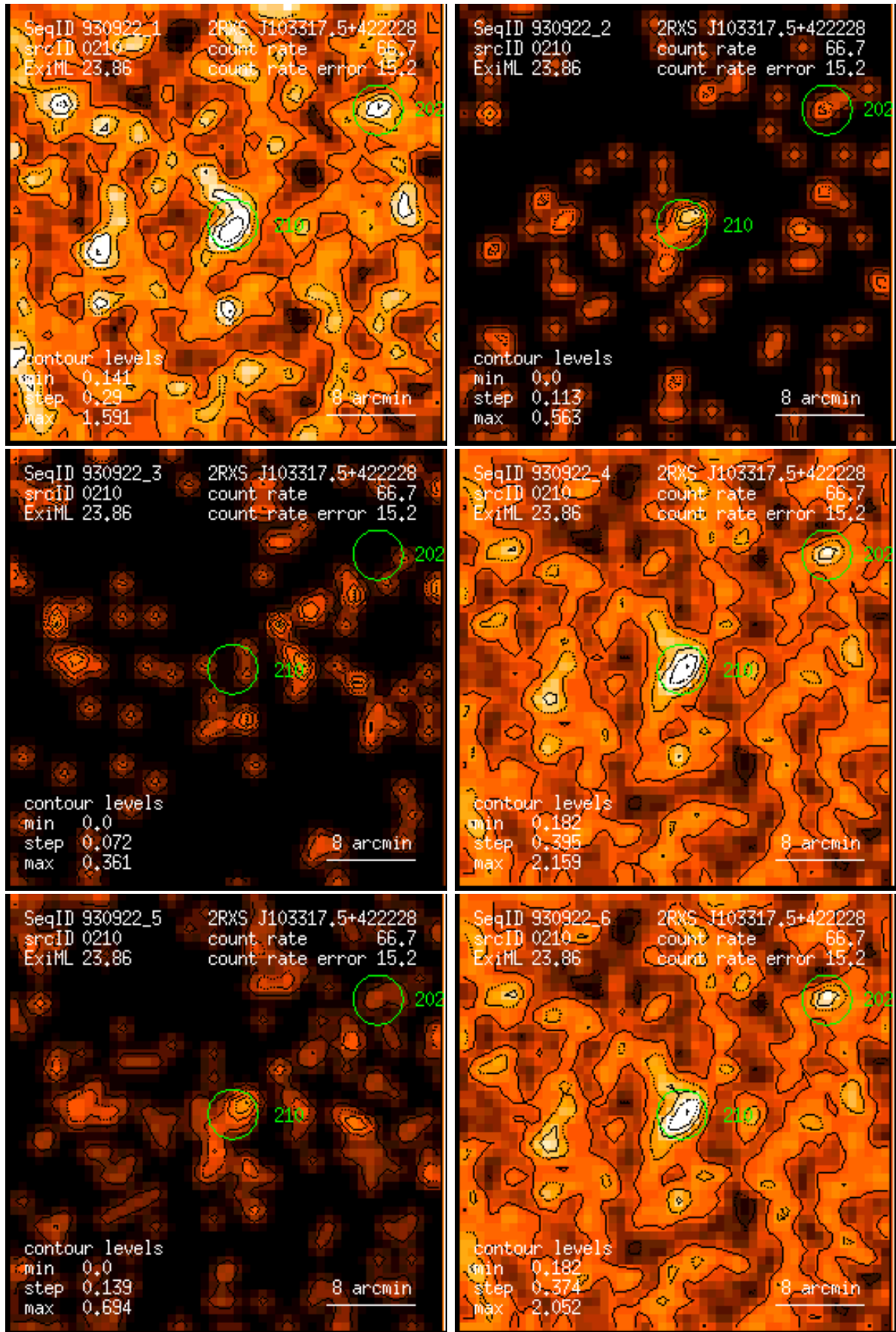
Figure 210: RASS 930922: detection 0210: band rate images, Gaussian filter: (1) PSPC channels 11 – 41, (2) 52 – 90, (3) 91 – 201, (4) 11 – 235, (5) 52 – 201, (6) 11 – 201. Broad band rates in counts/ks. Band rate contour levels in counts/ks/arcmin 2 .
