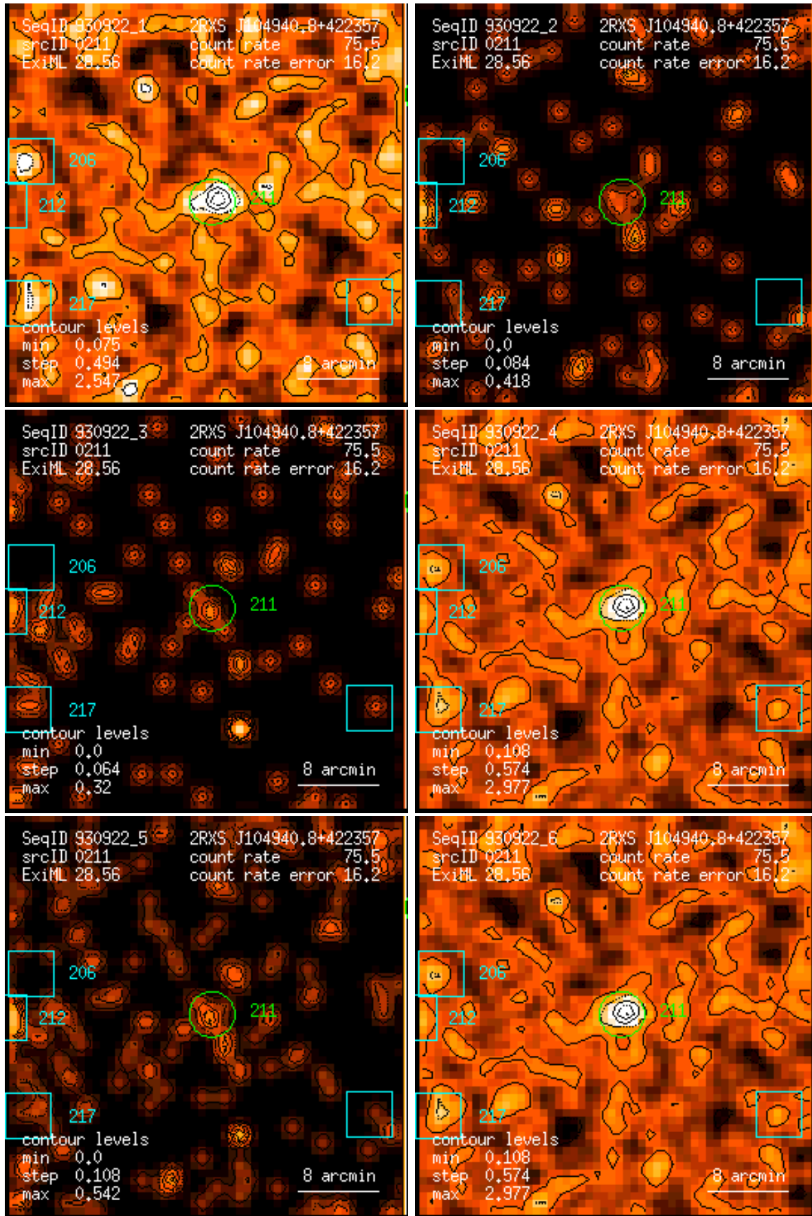
Figure 211: RASS 930922: detection 0211: band rate images, Gaussian filter: (1) PSPC channels 11 – 41, (2) 52 – 90, (3) 91 – 201, (4) 11 – 235, (5) 52 – 201, (6) 11 – 201. Broad band rates in counts/ks. Band rate contour levels in counts/ks/arcmin 2 .
