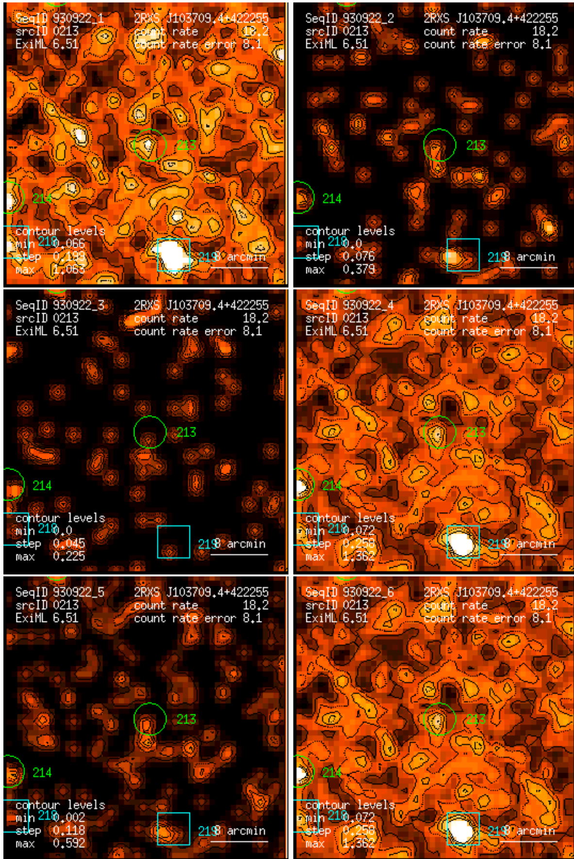
Figure 213: RASS 930922: detection 0213: band rate images, Gaussian filter: (1) PSPC channels 11 – 41, (2) 52 – 90, (3) 91 – 201, (4) 11 – 235, (5) 52 – 201, (6) 11 – 201. Broad band rates in counts/ks. Band rate contour levels in counts/ks/arcmin 2 .
