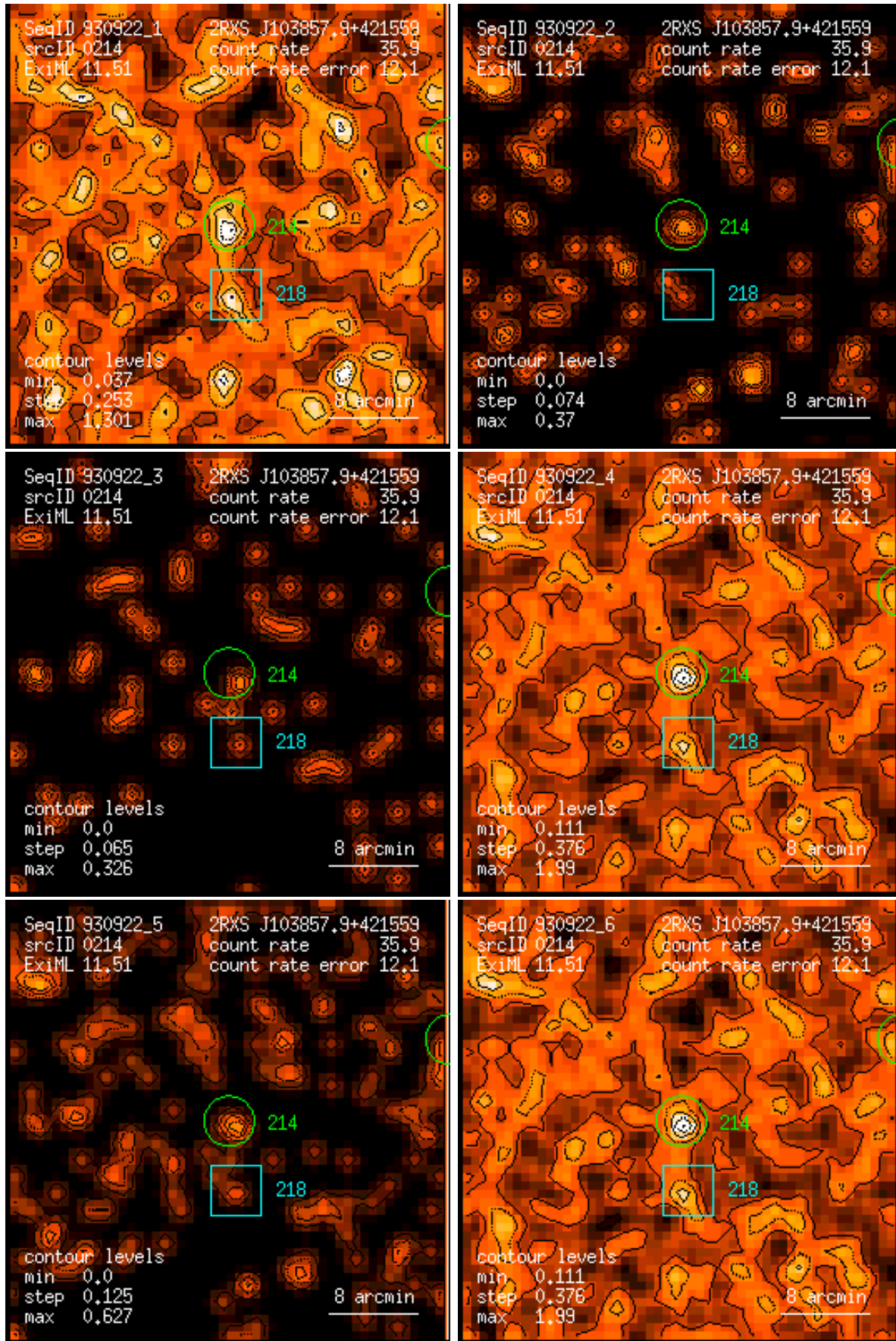
Figure 214: RASS 930922: detection 0214: band rate images, Gaussian filter: (1) PSPC channels 11 – 41, (2) 52 – 90, (3) 91 – 201, (4) 11 – 235, (5) 52 – 201, (6) 11 – 201. Broad band rates in counts/ks. Band rate contour levels in counts/ks/arcmin 2 .
