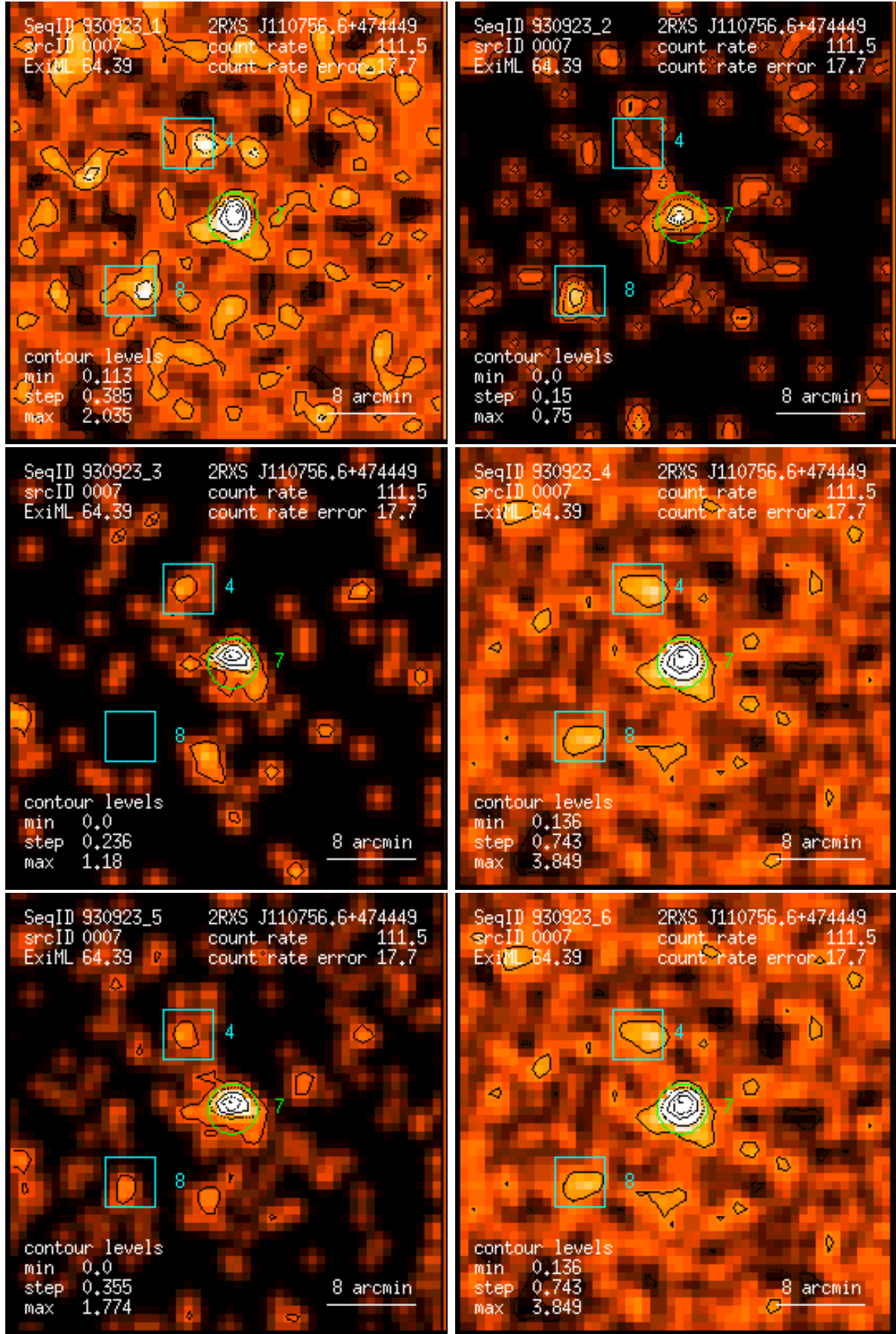
Figure 7: RASS 930923: detection 0007: band rate images, Gaussian filter: (1) PSPC channels 11 – 41, (2) 52 – 90, (3) 91 – 201, (4) 11 – 235, (5) 52 – 201, (6) 11 – 201. Broad band rates in counts/ks. Band rate contour levels in counts/ks/arcmin 2 .
