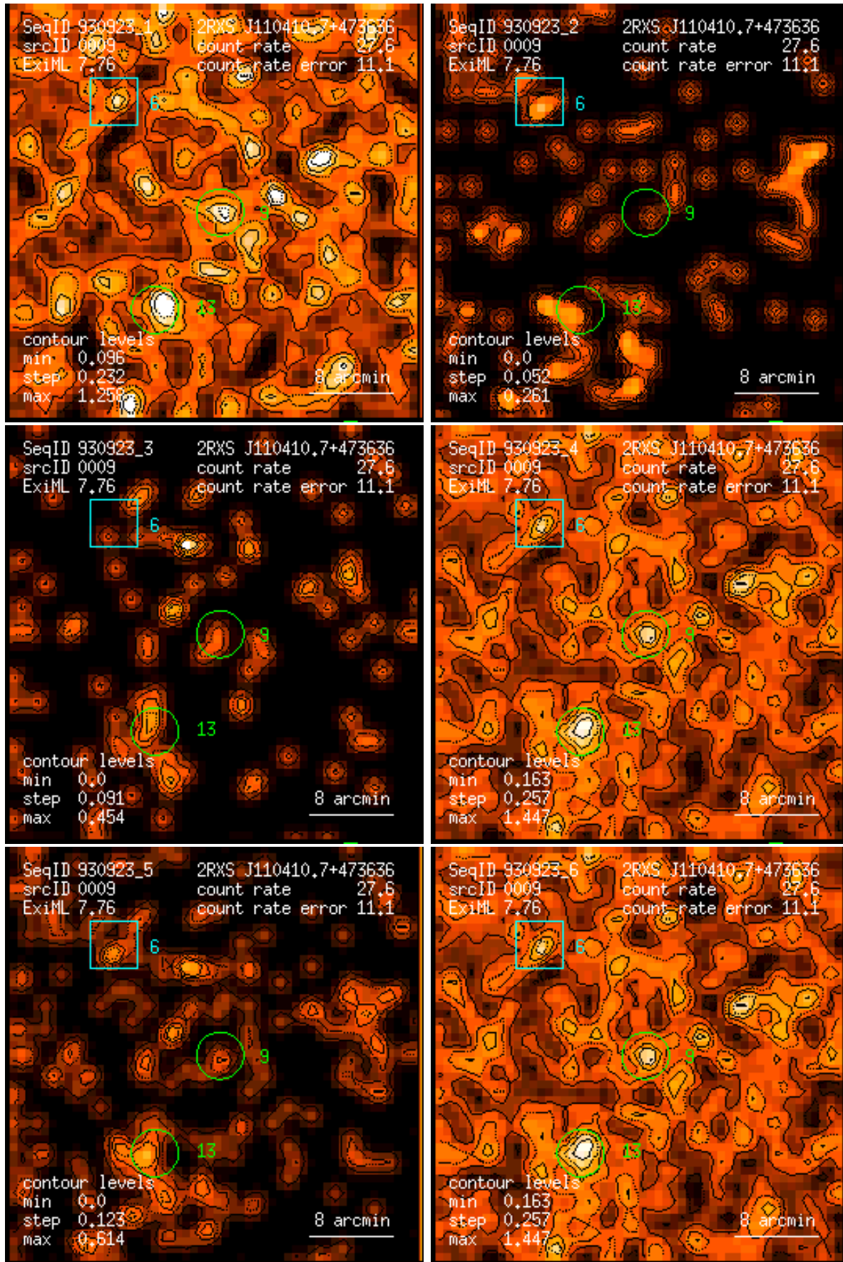
Figure 9: RASS 930923: detection 0009: band rate images, Gaussian filter: (1) PSPC channels 11 – 41, (2) 52 – 90, (3) 91 – 201, (4) 11 – 235, (5) 52 – 201, (6) 11 – 201. Broad band rates in counts/ks. Band rate contour levels in counts/ks/arcmin 2 .
