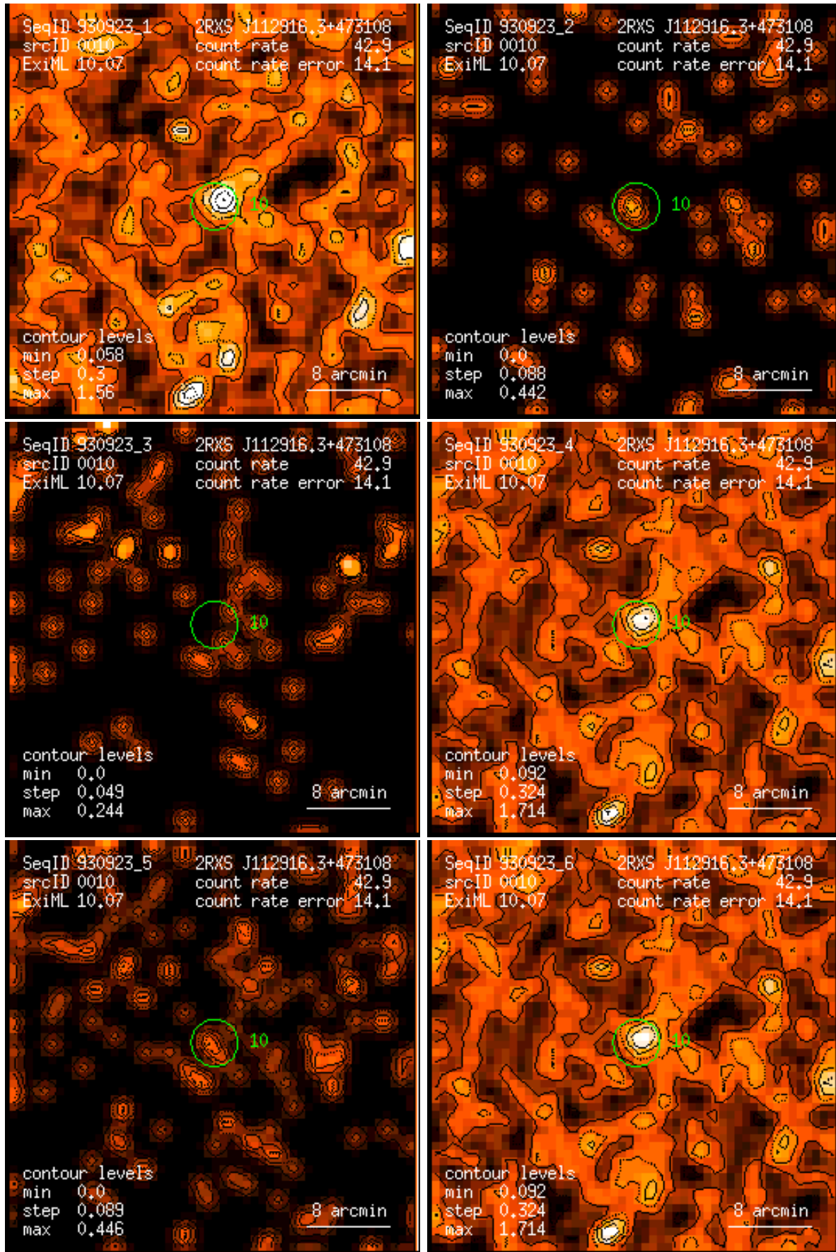
Figure 10: RASS 930923: detection 0010: band rate images, Gaussian filter: (1) PSPC channels 11 – 41, (2) 52 – 90, (3) 91 – 201, (4) 11 – 235, (5) 52 – 201, (6) 11 – 201. Broad band rates in counts/ks. Band rate contour levels in counts/ks/arcmin 2 .
