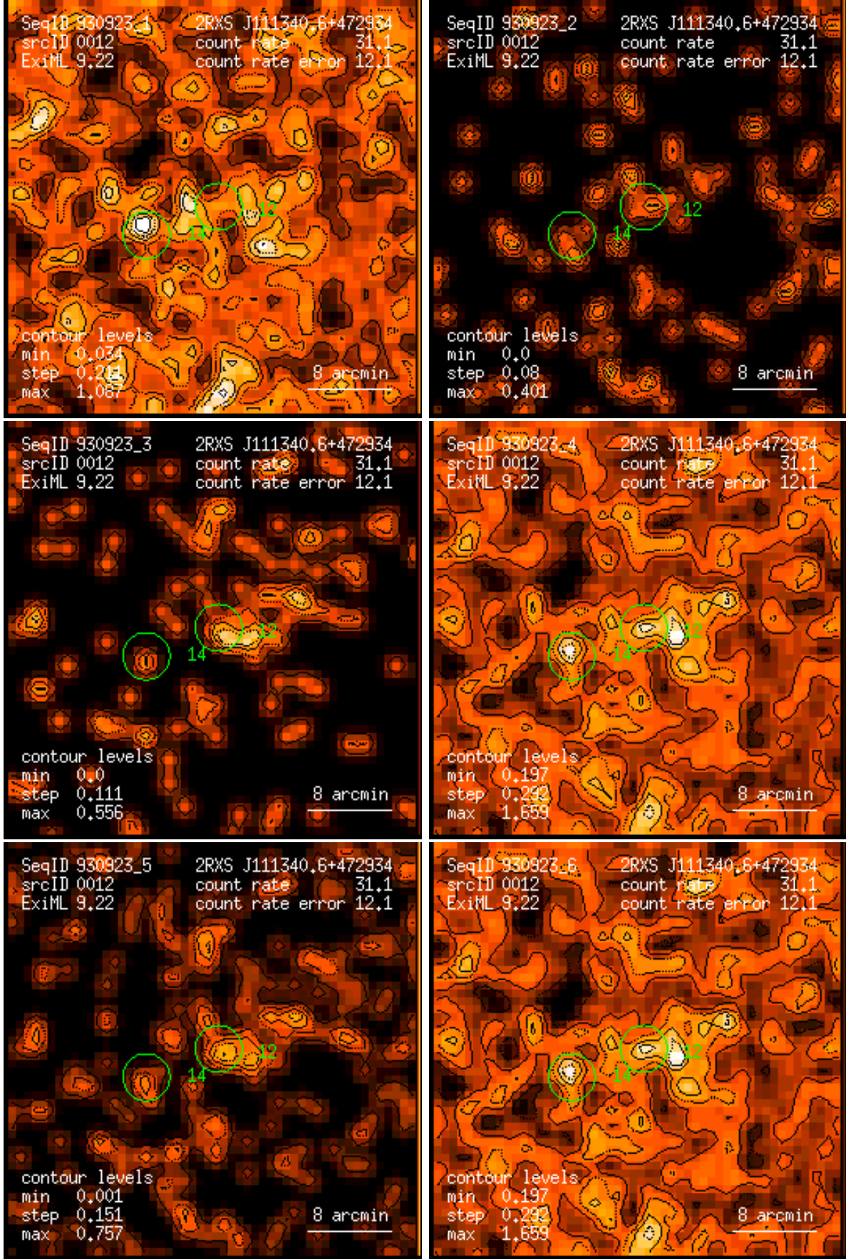
Figure 12: RASS 930923: detection 0012: band rate images, Gaussian filter: (1) PSPC channels 11 – 41, (2) 52 – 90, (3) 91 – 201, (4) 11 – 235, (5) 52 – 201, (6) 11 – 201. Broad band rates in counts/ks. Band rate contour levels in counts/ks/arcmin 2 .
