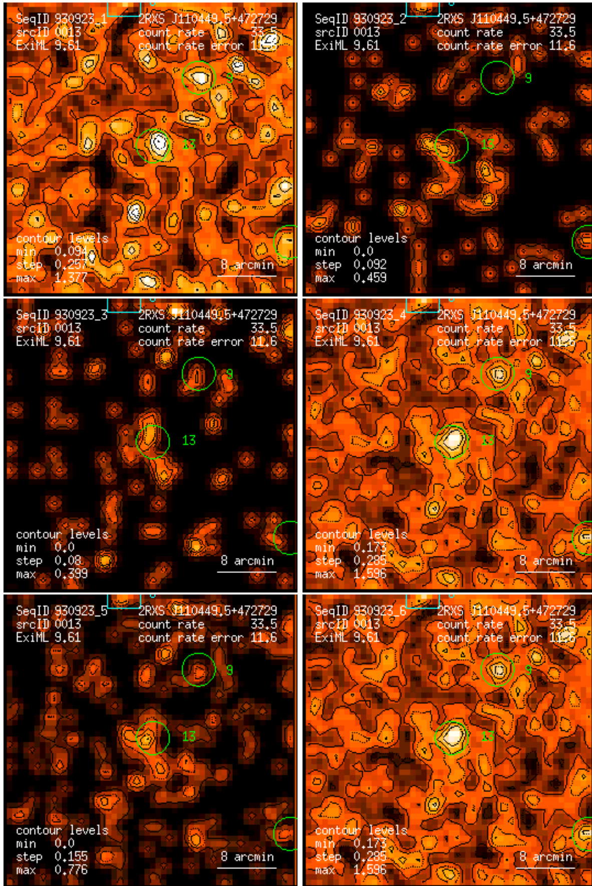
Figure 13: RASS 930923: detection 0013: band rate images, Gaussian filter: (1) PSPC channels 11 – 41, (2) 52 – 90, (3) 91 – 201, (4) 11 – 235, (5) 52 – 201, (6) 11 – 201. Broad band rates in counts/ks. Band rate contour levels in counts/ks/arcmin 2 .
