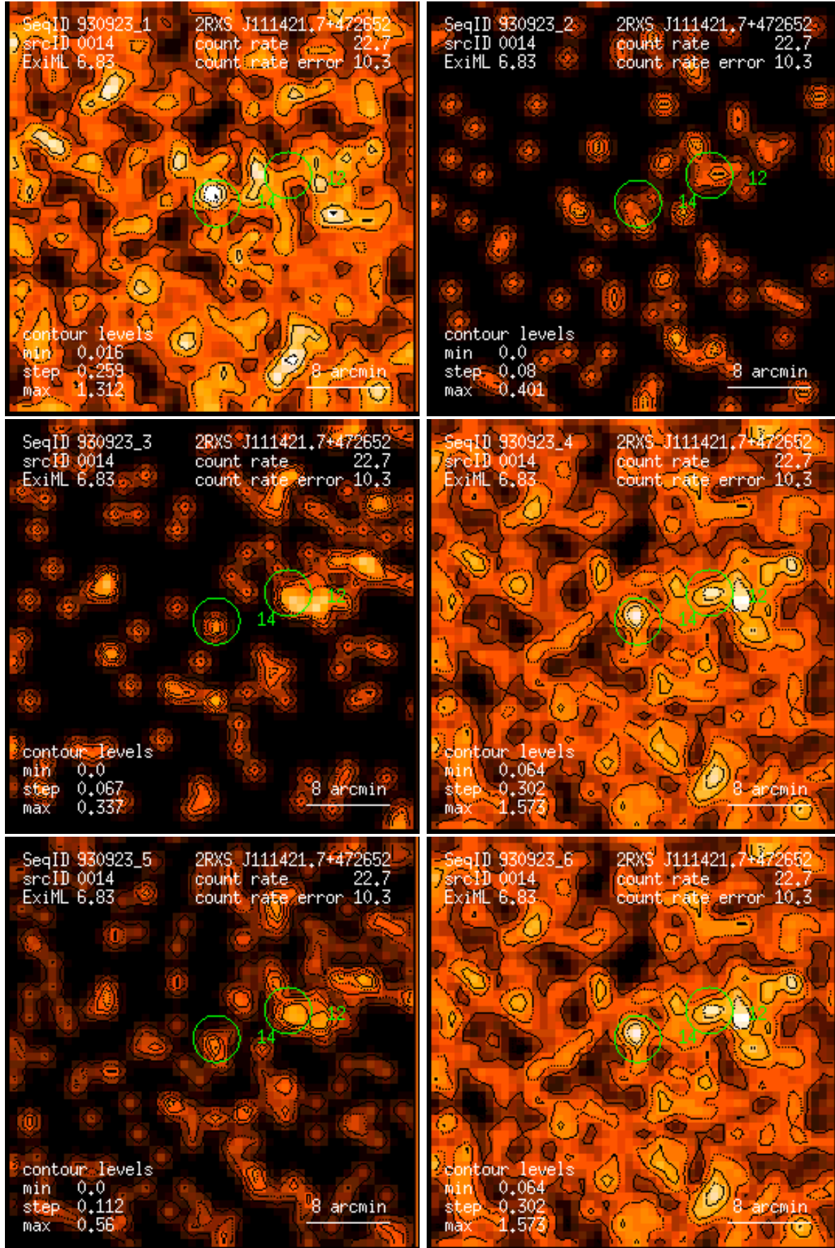
Figure 14: RASS 930923: detection 0014: band rate images, Gaussian filter: (1) PSPC channels 11 – 41, (2) 52 – 90, (3) 91 – 201, (4) 11 – 235, (5) 52 – 201, (6) 11 – 201. Broad band rates in counts/ks. Band rate contour levels in counts/ks/arcmin 2 .
