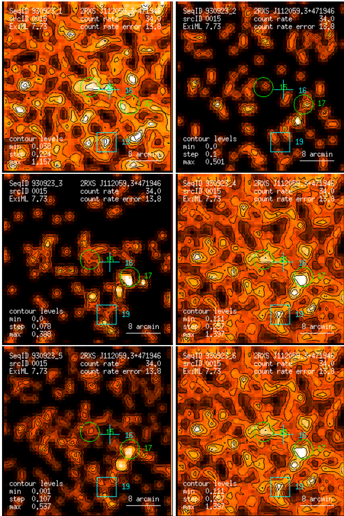
Figure 15: RASS 930923: detection 0015: band rate images, Gaussian filter: (1) PSPC channels 11 – 41, (2) 52 – 90, (3) 91 – 201, (4) 11 – 235, (5) 52 – 201, (6) 11 – 201. Broad band rates in counts/ks. Band rate contour levels in counts/ks/arcmin 2 .
