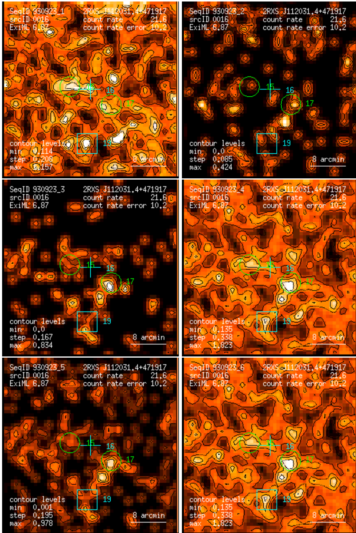
Figure 16: RASS 930923: detection 0016: band rate images, Gaussian filter: (1) PSPC channels 11 – 41, (2) 52 – 90, (3) 91 – 201, (4) 11 – 235, (5) 52 – 201, (6) 11 – 201. Broad band rates in counts/ks. Band rate contour levels in counts/ks/arcmin 2 .
