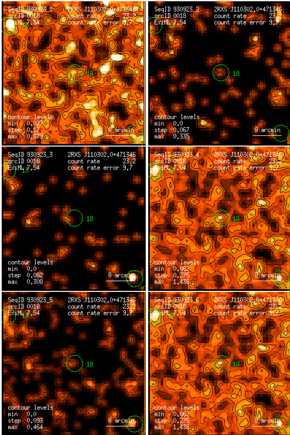
Figure 18: RASS 930923: detection 0018: band rate images, Gaussian filter: (1) PSPC channels 11 – 41, (2) 52 – 90, (3) 91 – 201, (4) 11 – 235, (5) 52 – 201, (6) 11 – 201. Broad band rates in counts/ks. Band rate contour levels in counts/ks/arcmin 2 .
