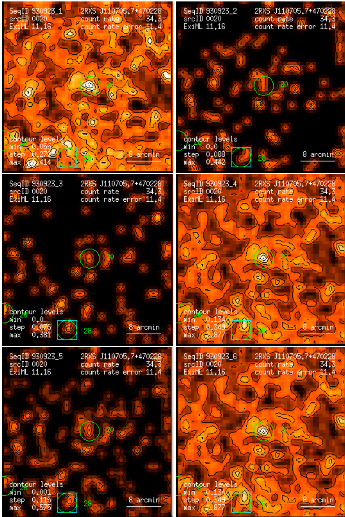
Figure 20: RASS 930923: detection 0020: band rate images, Gaussian filter: (1) PSPC channels 11 – 41, (2) 52 – 90, (3) 91 – 201, (4) 11 – 235, (5) 52 – 201, (6) 11 – 201. Broad band rates in counts/ks. Band rate contour levels in counts/ks/arcmin 2 .
