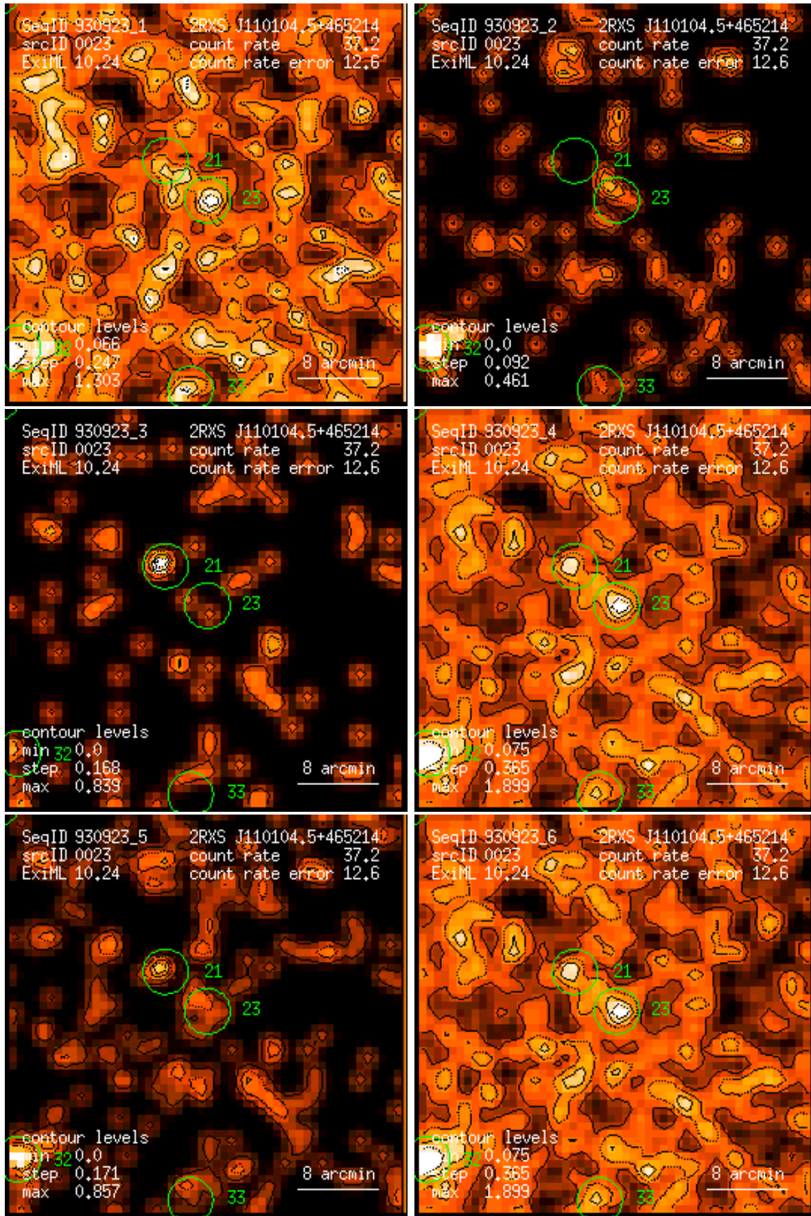
Figure 23: RASS 930923: detection 0023: band rate images, Gaussian filter: (1) PSPC channels 11 – 41, (2) 52 – 90, (3) 91 – 201, (4) 11 – 235, (5) 52 – 201, (6) 11 – 201. Broad band rates in counts/ks. Band rate contour levels in counts/ks/arcmin 2 .
