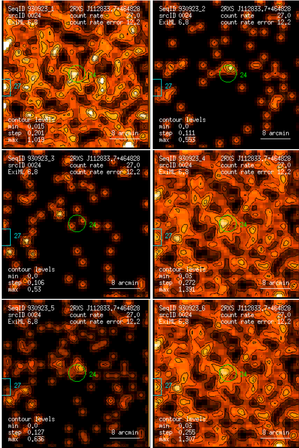
Figure 24: RASS 930923: detection 0024: band rate images, Gaussian filter: (1) PSPC channels 11 – 41, (2) 52 – 90, (3) 91 – 201, (4) 11 – 235, (5) 52 – 201, (6) 11 – 201. Broad band rates in counts/ks. Band rate contour levels in counts/ks/arcmin 2 .
