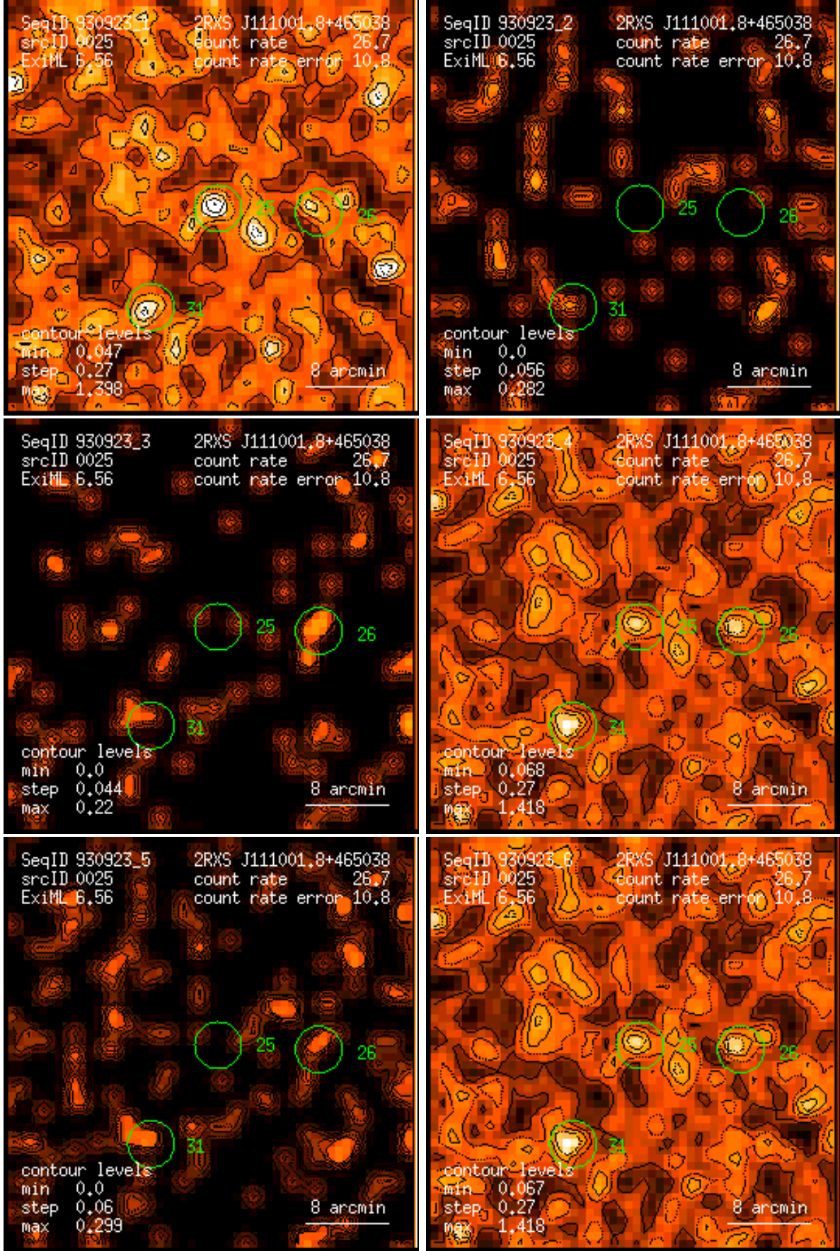
Figure 25: RASS 930923: detection 0025: band rate images, Gaussian filter: (1) PSPC channels 11 – 41, (2) 52 – 90, (3) 91 – 201, (4) 11 – 235, (5) 52 – 201, (6) 11 – 201. Broad band rates in counts/ks. Band rate contour levels in counts/ks/arcmin 2 .
