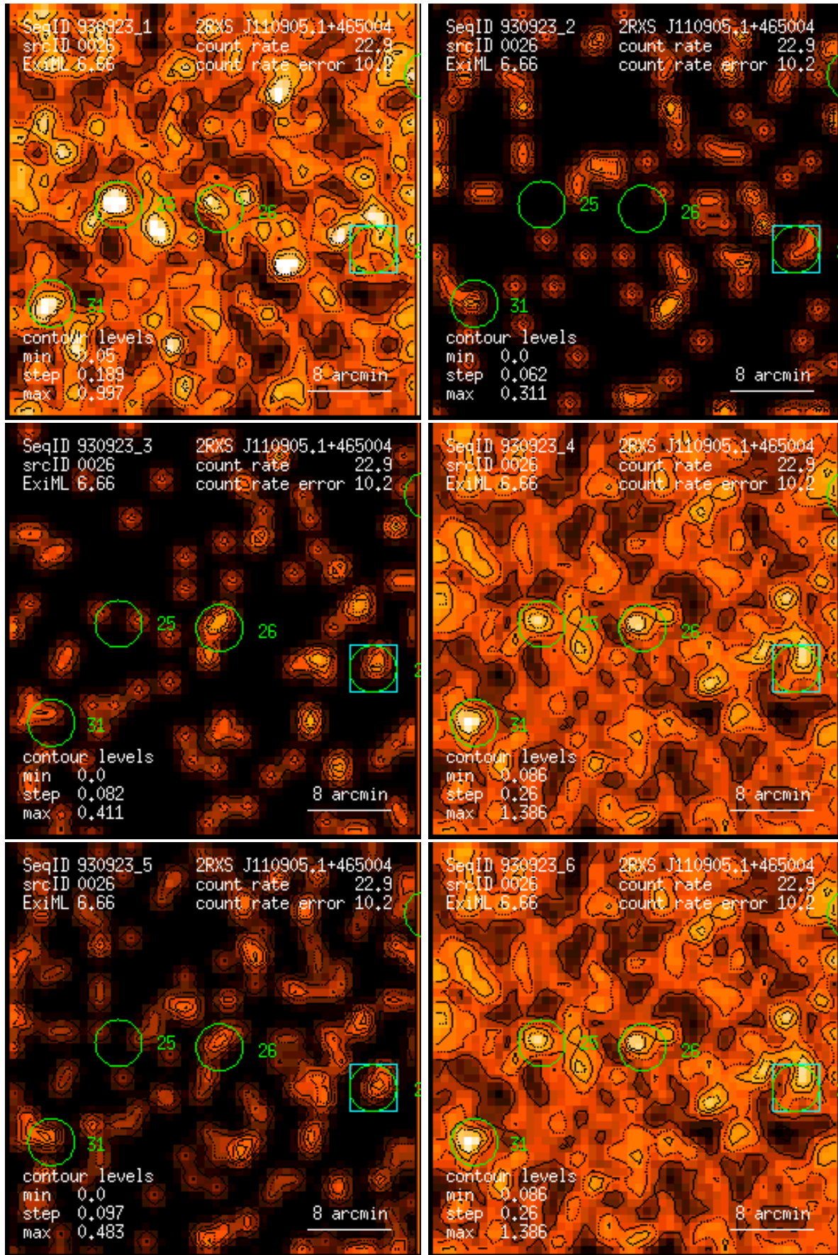
Figure 26: RASS 930923: detection 0026: band rate images, Gaussian filter: (1) PSPC channels 11 – 41, (2) 52 – 90, (3) 91 – 201, (4) 11 – 235, (5) 52 – 201, (6) 11 – 201. Broad band rates in counts/ks. Band rate contour levels in counts/ks/arcmin 2 .
