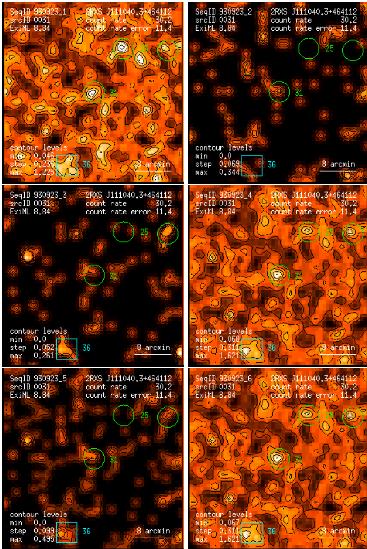
Figure 31: RASS 930923: detection 0031: band rate images, Gaussian filter: (1) PSPC channels 11 – 41, (2) 52 – 90, (3) 91 – 201, (4) 11 – 235, (5) 52 – 201, (6) 11 – 201. Broad band rates in counts/ks. Band rate contour levels in counts/ks/arcmin 2 .
