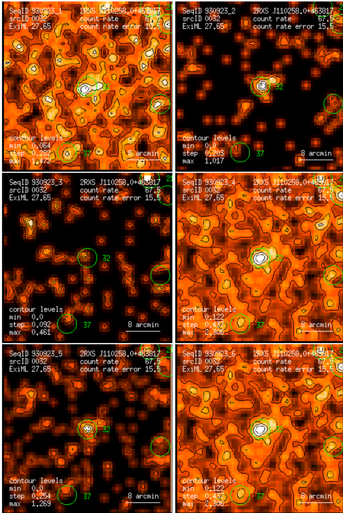
Figure 32: RASS 930923: detection 0032: band rate images, Gaussian filter: (1) PSPC channels 11 – 41, (2) 52 – 90, (3) 91 – 201, (4) 11 – 235, (5) 52 – 201, (6) 11 – 201. Broad band rates in counts/ks. Band rate contour levels in counts/ks/arcmin 2 .
