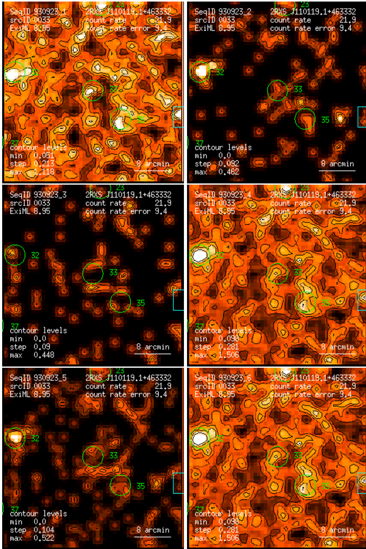
Figure 33: RASS 930923: detection 0033: band rate images, Gaussian filter: (1) PSPC channels 11 – 41, (2) 52 – 90, (3) 91 – 201, (4) 11 – 235, (5) 52 – 201, (6) 11 – 201. Broad band rates in counts/ks. Band rate contour levels in counts/ks/arcmin 2 .
