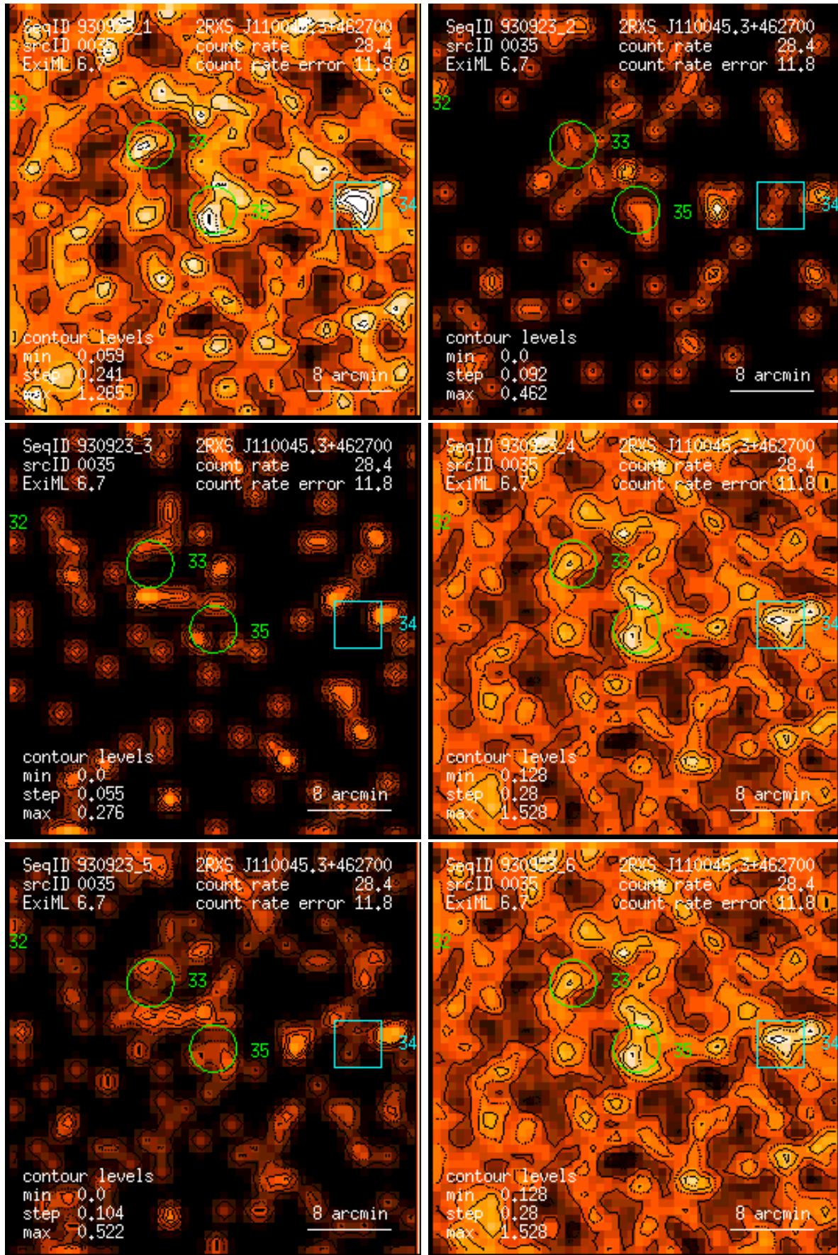
Figure 35: RASS 930923: detection 0035: band rate images, Gaussian filter: (1) PSPC channels 11 – 41, (2) 52 – 90, (3) 91 – 201, (4) 11 – 235, (5) 52 – 201, (6) 11 – 201. Broad band rates in counts/ks. Band rate contour levels in counts/ks/arcmin 2 .
