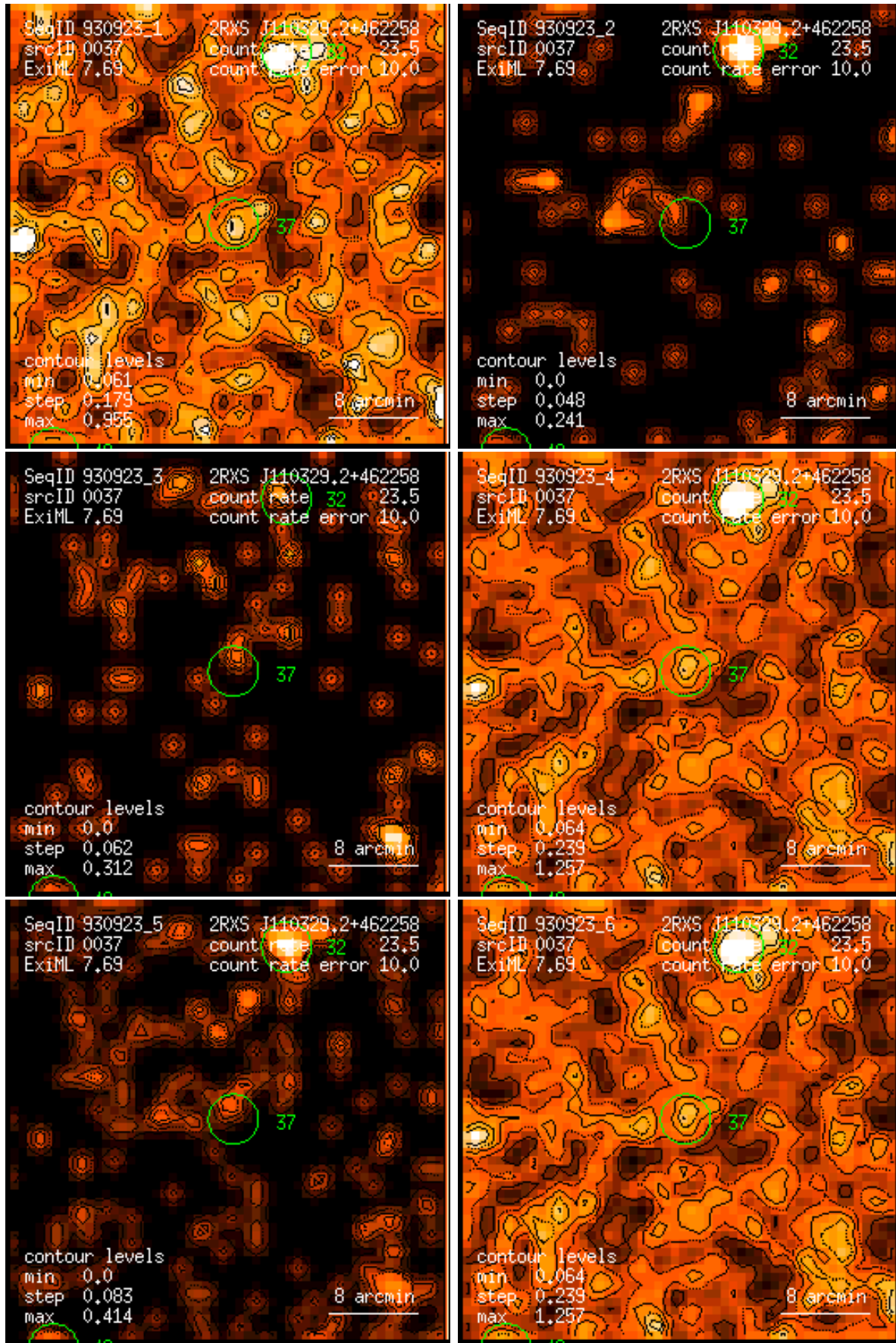
Figure 37: RASS 930923: detection 0037: band rate images, Gaussian filter: (1) PSPC channels 11 – 41, (2) 52 – 90, (3) 91 – 201, (4) 11 – 235, (5) 52 – 201, (6) 11 – 201. Broad band rates in counts/ks. Band rate contour levels in counts/ks/arcmin 2 .
