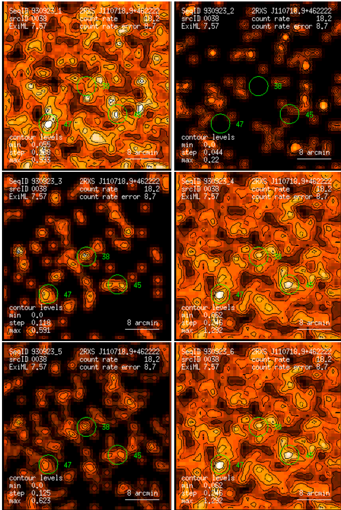
Figure 38: RASS 930923: detection 0038: band rate images, Gaussian filter: (1) PSPC channels 11 – 41, (2) 52 – 90, (3) 91 – 201, (4) 11 – 235, (5) 52 – 201, (6) 11 – 201. Broad band rates in counts/ks. Band rate contour levels in counts/ks/arcmin 2 .
