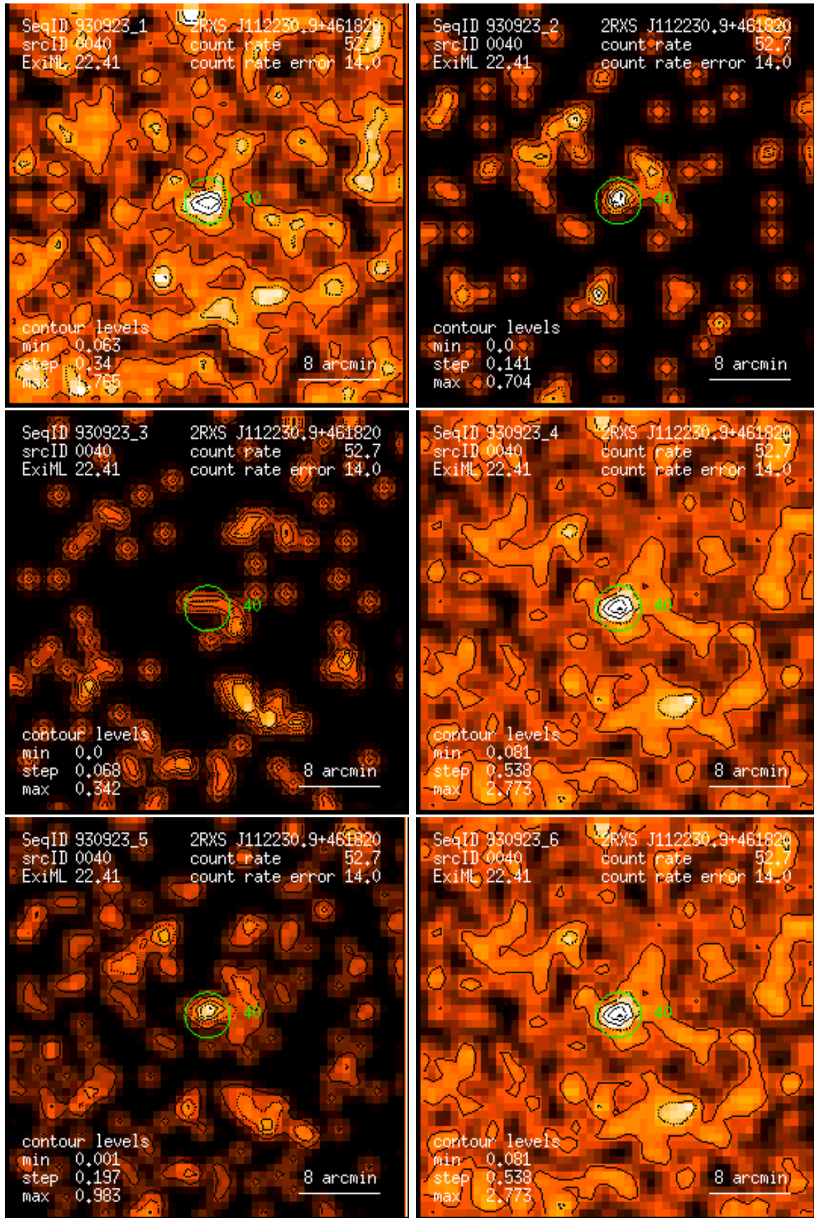
Figure 40: RASS 930923: detection 0040: band rate images, Gaussian filter: (1) PSPC channels 11 – 41, (2) 52 – 90, (3) 91 – 201, (4) 11 – 235, (5) 52 – 201, (6) 11 – 201. Broad band rates in counts/ks. Band rate contour levels in counts/ks/arcmin 2 .
