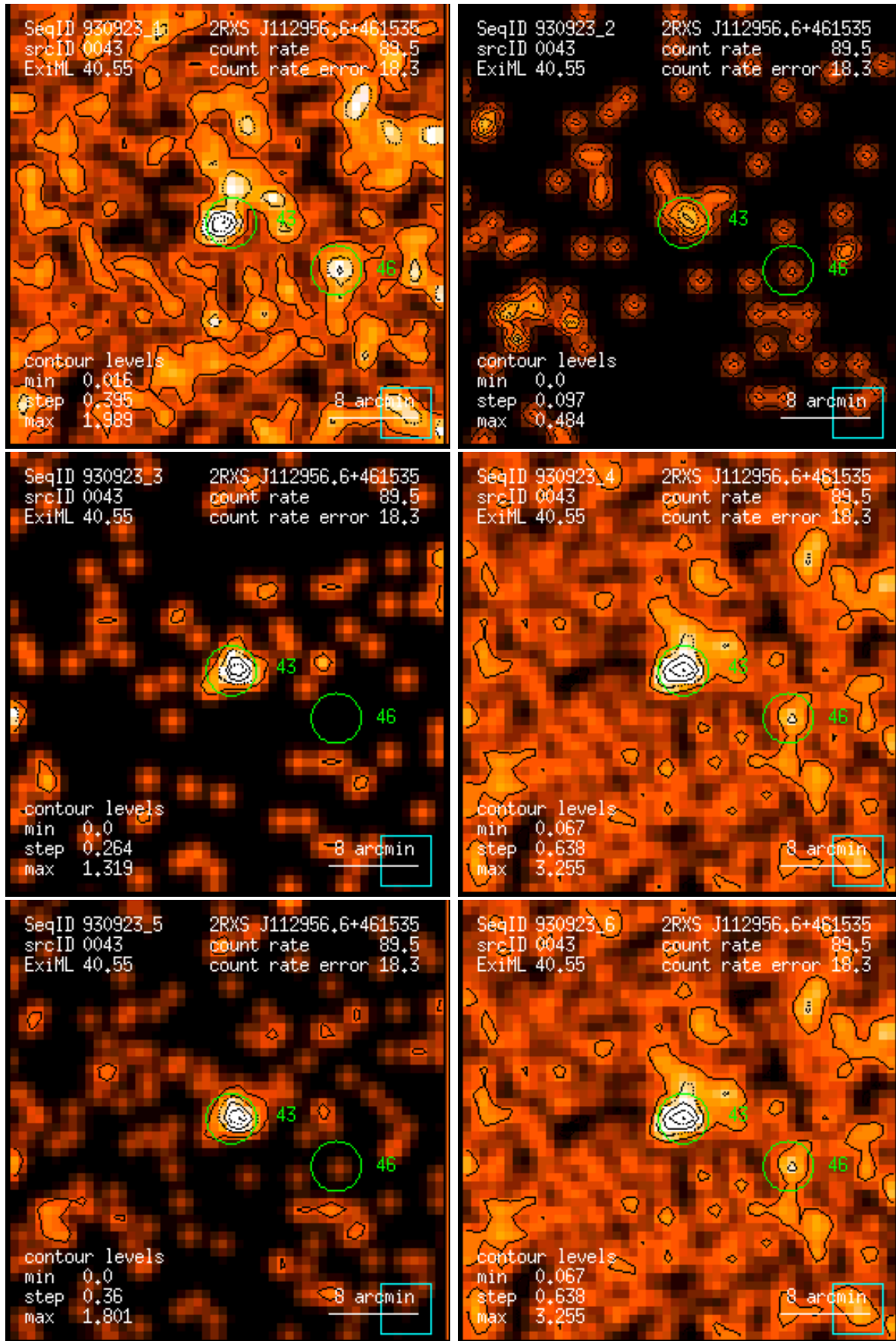
Figure 43: RASS 930923: detection 0043: band rate images, Gaussian filter: (1) PSPC channels 11 – 41, (2) 52 – 90, (3) 91 – 201, (4) 11 – 235, (5) 52 – 201, (6) 11 – 201. Broad band rates in counts/ks. Band rate contour levels in counts/ks/arcmin 2 .
