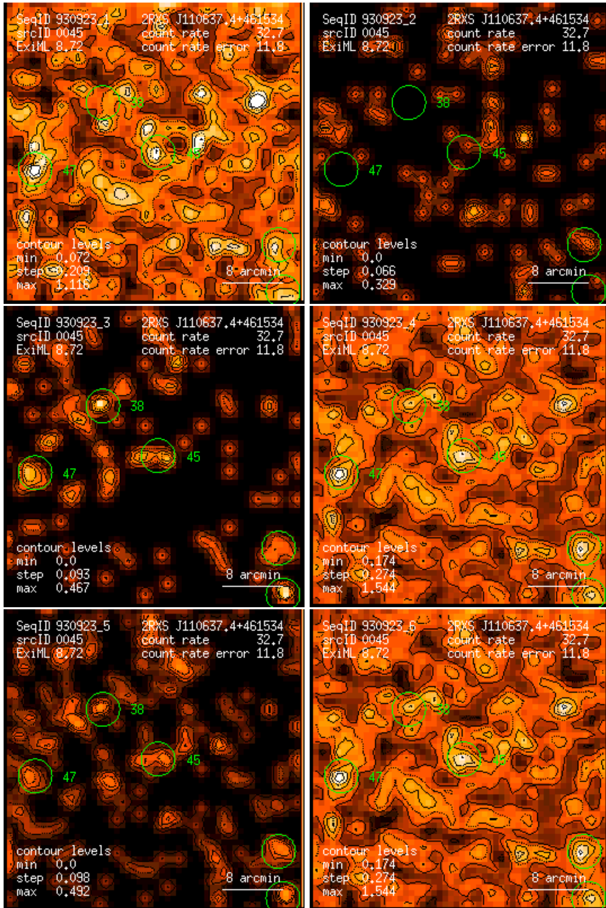
Figure 45: RASS 930923: detection 0045: band rate images, Gaussian filter: (1) PSPC channels 11 – 41, (2) 52 – 90, (3) 91 – 201, (4) 11 – 235, (5) 52 – 201, (6) 11 – 201. Broad band rates in counts/ks. Band rate contour levels in counts/ks/arcmin 2 .
