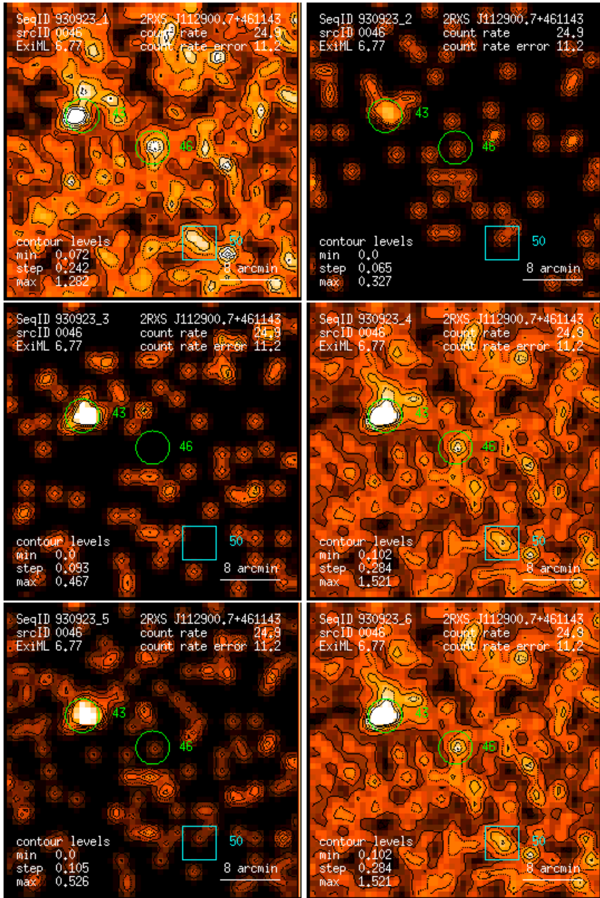
Figure 46: RASS 930923: detection 0046: band rate images, Gaussian filter: (1) PSPC channels 11 – 41, (2) 52 – 90, (3) 91 – 201, (4) 11 – 235, (5) 52 – 201, (6) 11 – 201. Broad band rates in counts/ks. Band rate contour levels in counts/ks/arcmin 2 .
