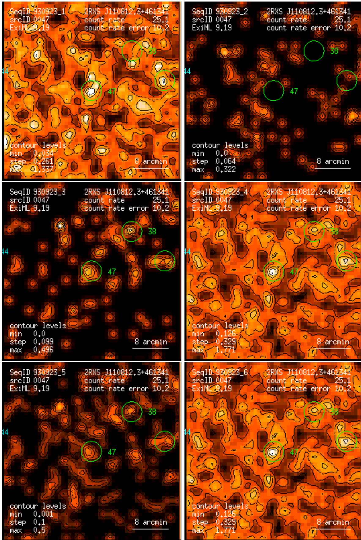
Figure 47: RASS 930923: detection 0047: band rate images, Gaussian filter: (1) PSPC channels 11 – 41, (2) 52 – 90, (3) 91 – 201, (4) 11 – 235, (5) 52 – 201, (6) 11 – 201. Broad band rates in counts/ks. Band rate contour levels in counts/ks/arcmin 2 .
