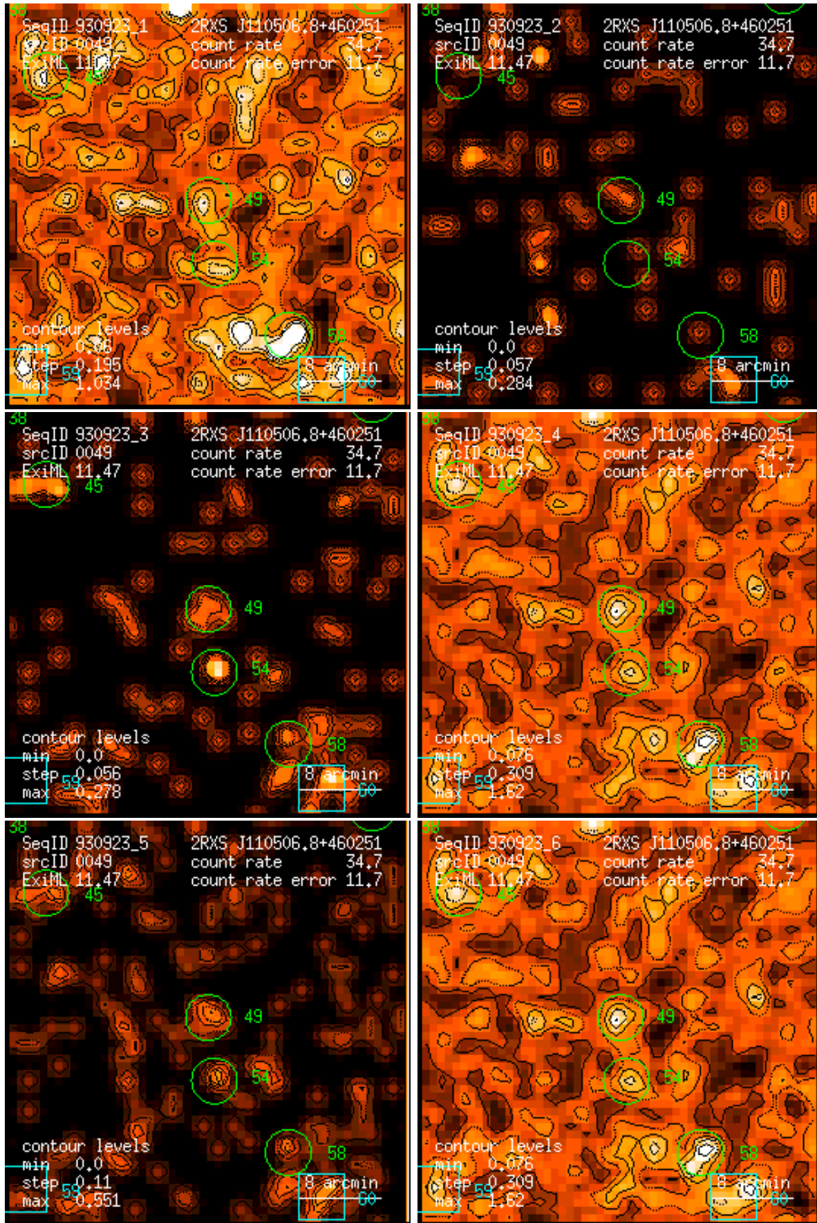
Figure 49: RASS 930923: detection 0049: band rate images, Gaussian filter: (1) PSPC channels 11 – 41, (2) 52 – 90, (3) 91 – 201, (4) 11 – 235, (5) 52 – 201, (6) 11 – 201. Broad band rates in counts/ks. Band rate contour levels in counts/ks/arcmin 2 .
