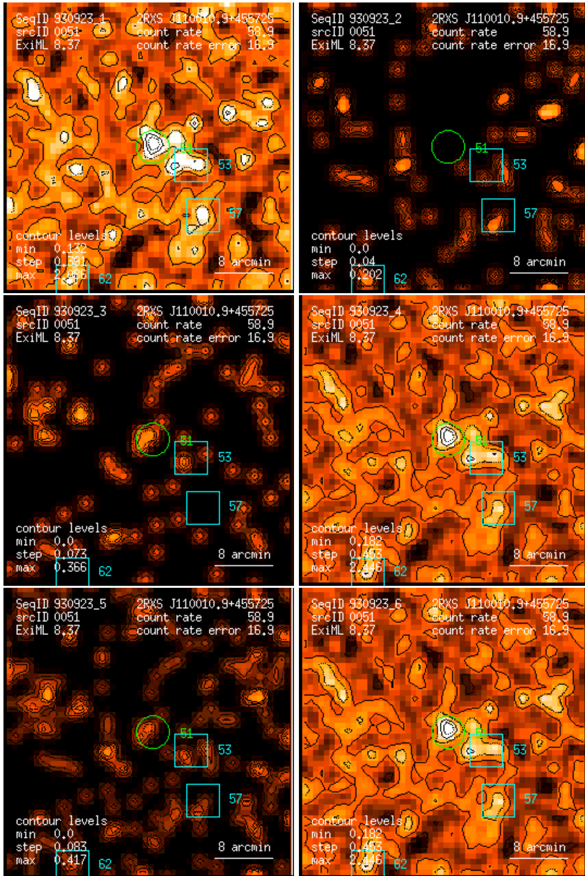
Figure 51: RASS 930923: detection 0051: band rate images, Gaussian filter: (1) PSPC channels 11 – 41, (2) 52 – 90, (3) 91 – 201, (4) 11 – 235, (5) 52 – 201, (6) 11 – 201. Broad band rates in counts/ks. Band rate contour levels in counts/ks/arcmin 2 .
