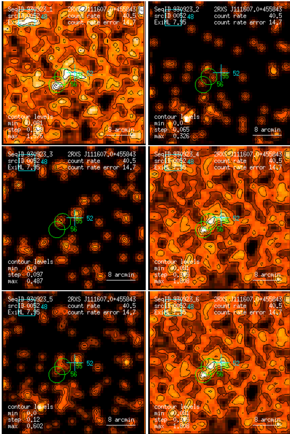
Figure 52: RASS 930923: detection 0052: band rate images, Gaussian filter: (1) PSPC channels 11 – 41, (2) 52 – 90, (3) 91 – 201, (4) 11 – 235, (5) 52 – 201, (6) 11 – 201. Broad band rates in counts/ks. Band rate contour levels in counts/ks/arcmin 2 .
