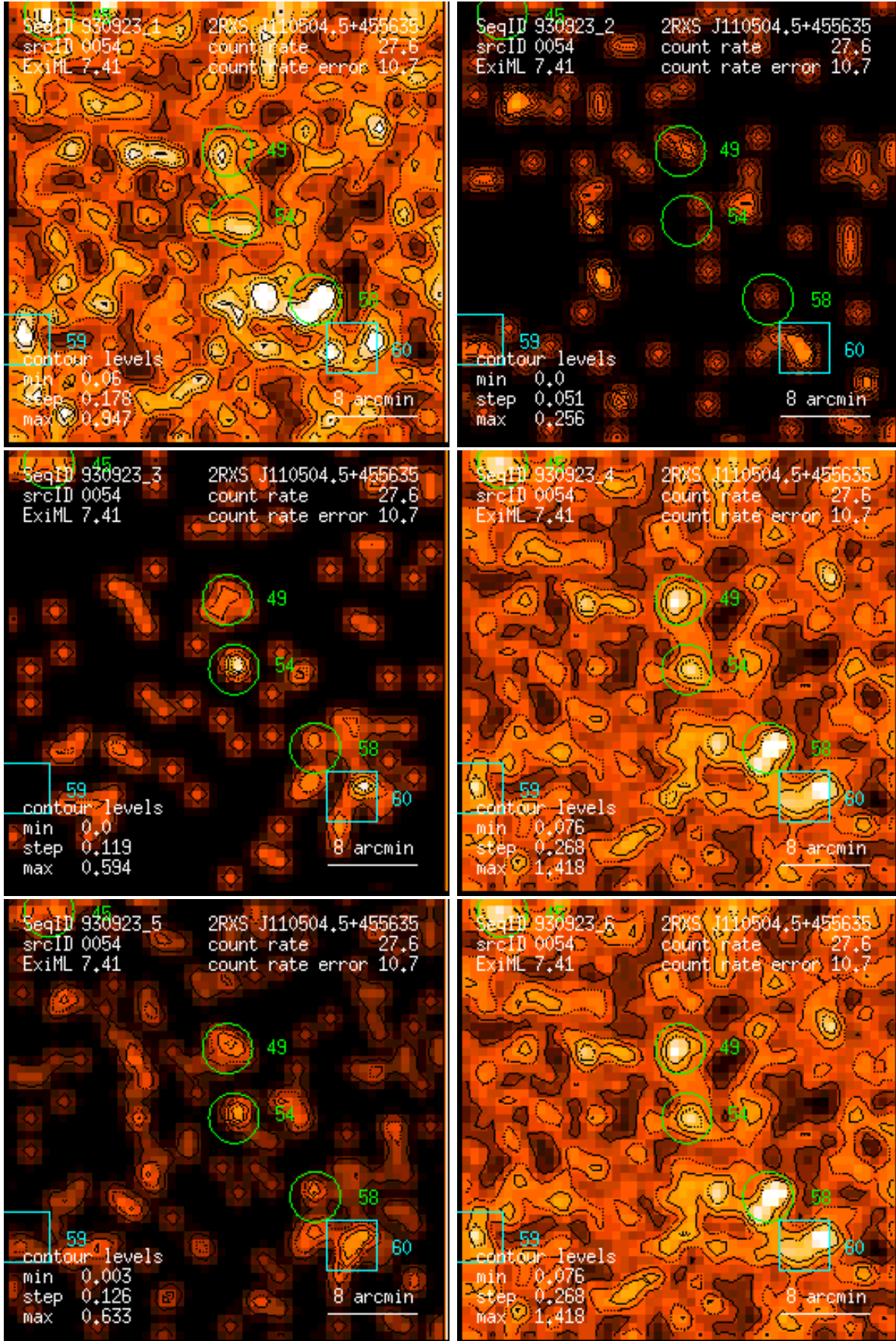
Figure 54: RASS 930923: detection 0054: band rate images, Gaussian filter: (1) PSPC channels 11 – 41, (2) 52 – 90, (3) 91 – 201, (4) 11 – 235, (5) 52 – 201, (6) 11 – 201. Broad band rates in counts/ks. Band rate contour levels in counts/ks/arcmin 2 .
