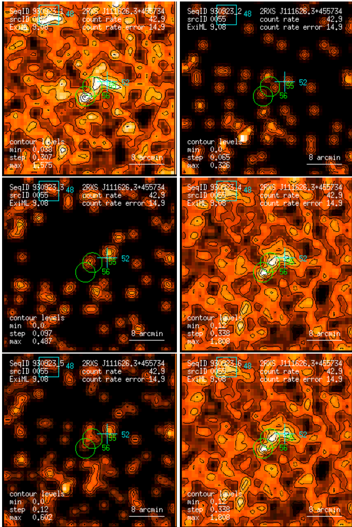
Figure 55: RASS 930923: detection 0055: band rate images, Gaussian filter: (1) PSPC channels 11 – 41, (2) 52 – 90, (3) 91 – 201, (4) 11 – 235, (5) 52 – 201, (6) 11 – 201. Broad band rates in counts/ks. Band rate contour levels in counts/ks/arcmin 2 .
