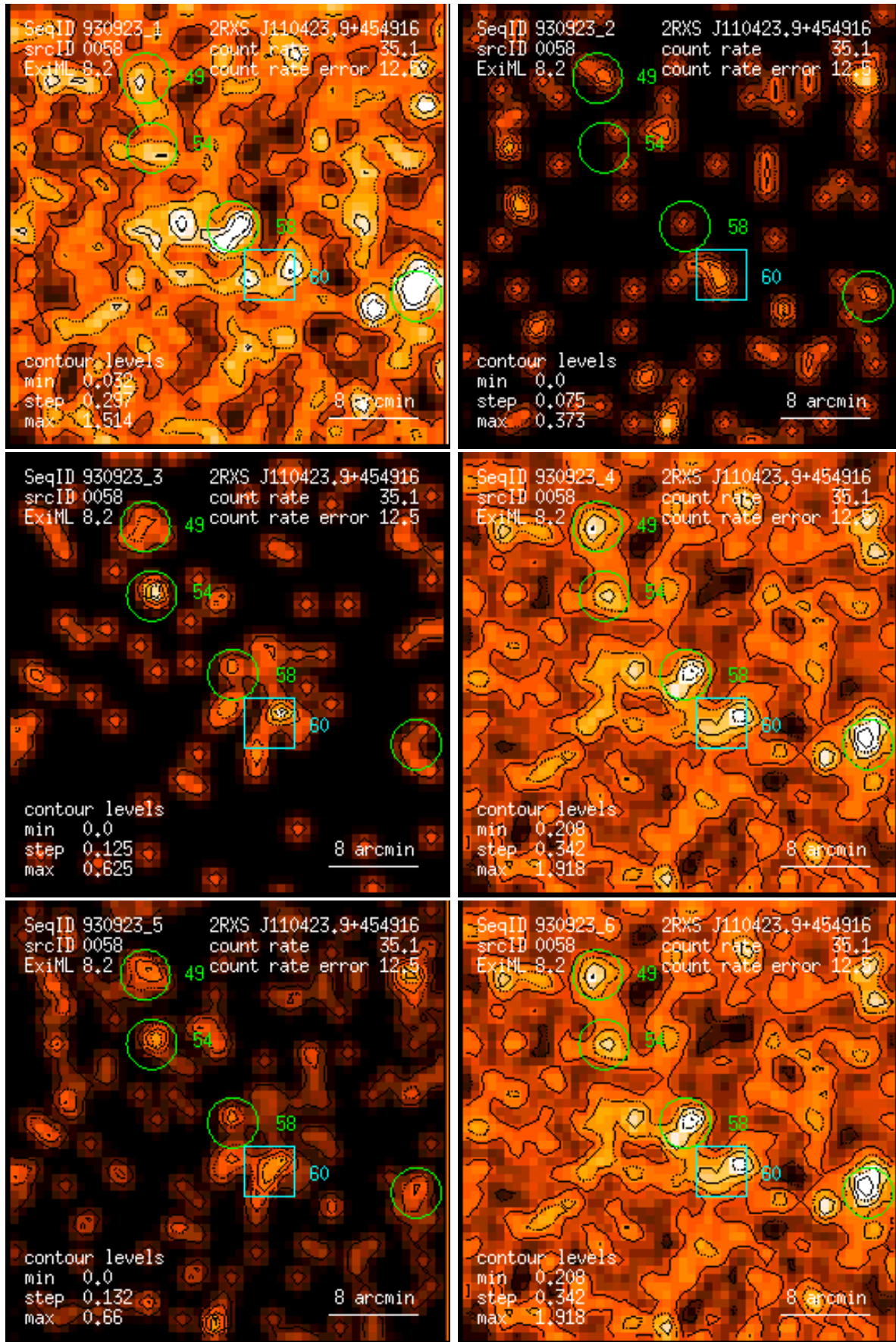
Figure 58: RASS 930923: detection 0058: band rate images, Gaussian filter: (1) PSPC channels 11 – 41, (2) 52 – 90, (3) 91 – 201, (4) 11 – 235, (5) 52 – 201, (6) 11 – 201. Broad band rates in counts/ks. Band rate contour levels in counts/ks/arcmin 2 .
