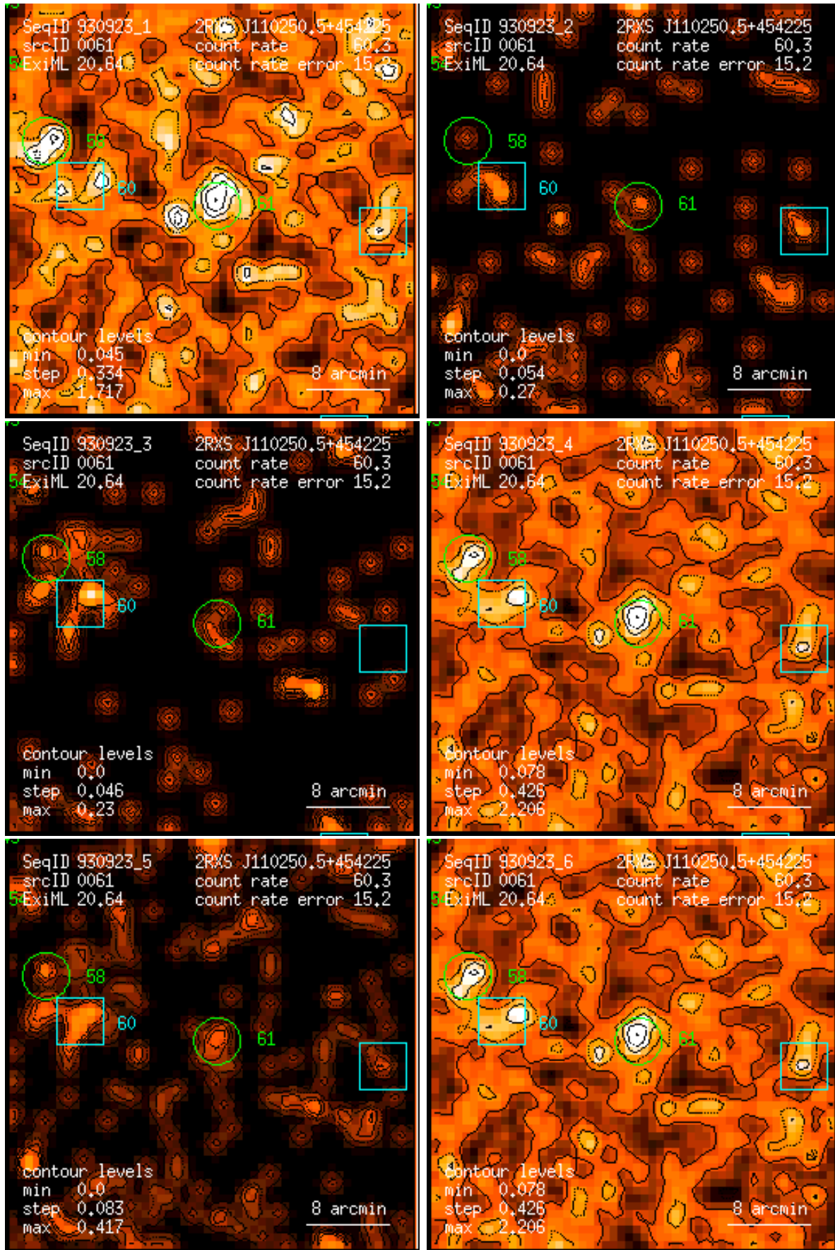
Figure 61: RASS 930923: detection 0061: band rate images, Gaussian filter: (1) PSPC channels 11 – 41, (2) 52 – 90, (3) 91 – 201, (4) 11 – 235, (5) 52 – 201, (6) 11 – 201. Broad band rates in counts/ks. Band rate contour levels in counts/ks/arcmin 2 .
