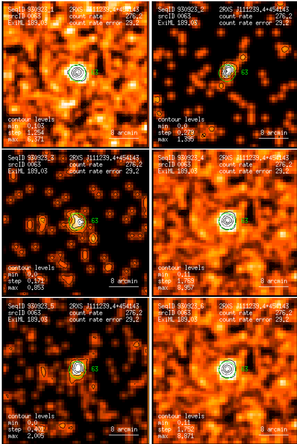
Figure 63: RASS 930923: detection 0063: band rate images, Gaussian filter: (1) PSPC channels 11 – 41, (2) 52 – 90, (3) 91 – 201, (4) 11 – 235, (5) 52 – 201, (6) 11 – 201. Broad band rates in counts/ks. Band rate contour levels in counts/ks/arcmin 2 .
